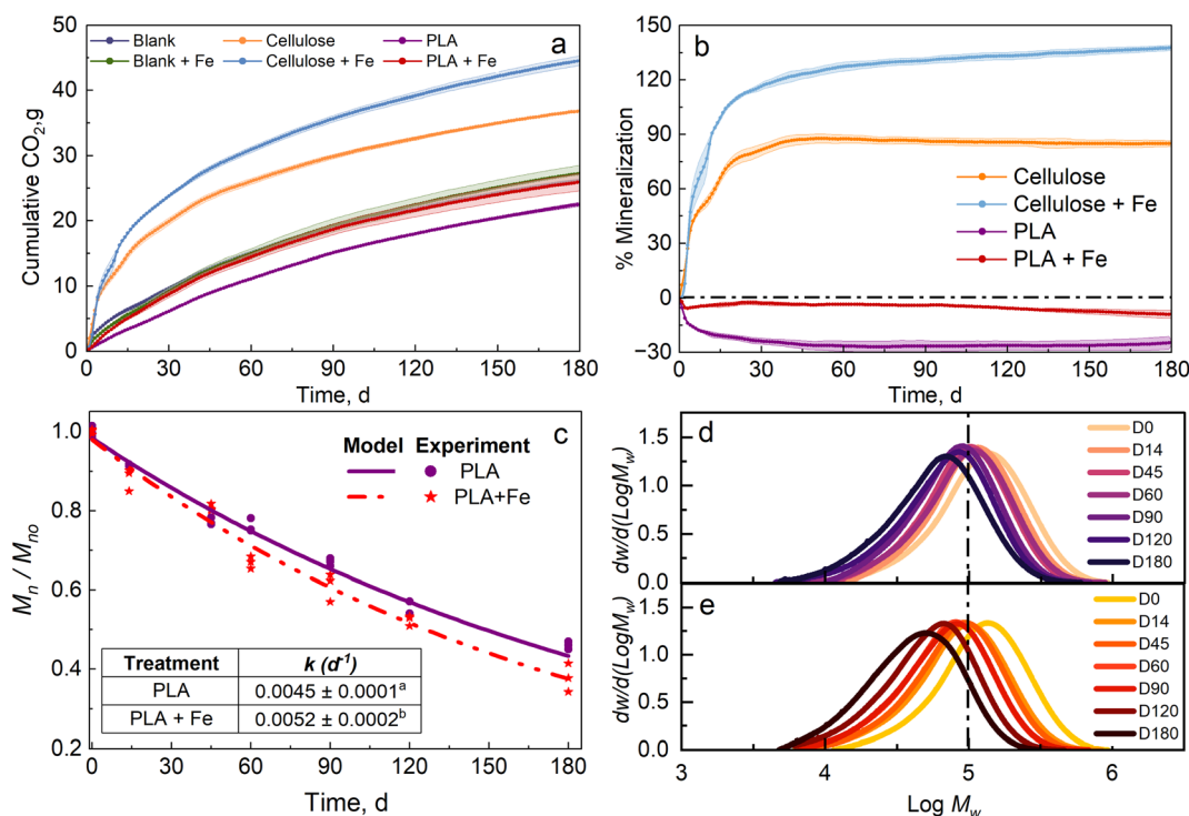
Fig. 1 Cumulative CO 2 evolution (a) and mineralization (b) of blank, cellulose, PLA, blank + Fe 3 O 4 (blank + Fe), cellulose + Fe 3 O 4 (cellulose + Fe), PLA + Fe 3 O 4 (PLA + Fe) in compost at 37 °C. (c) Represents the normalized M_n reduction as a function of time for PLA in control compost and compost biostimulated with Fe 3 O 4 . The experimental data was fitted using a first-order reaction of the form M_n/M_{n0} = e^{-kt} , where M_{n0} is the initial M_n , k is the rate constant, and t is the time. The inset shows the k -fitted values; values with different lowercase letters are statistically different ( \alpha = 0.05 , Tukey–Kramer test). (d) and (e) show the MWD of PLA in compost and compost biostimulated with Fe 3 O 4 , respectively.
