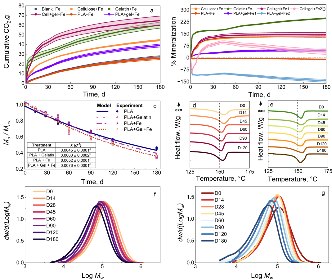
Fig. 3 Cumulative CO 2 evolution (a) and mineralization (b) of blank + Fe, cellulose + Fe, PLA + Fe, cellulose + gelatin + Fe, cellulose + gelatin + Fe, cellulose + gelatin + Fe (Cell + gel + Fe), PLA + gelatin + Fe (PLA + gel + Fe) in compost at 37 °C. (c) Represents the normalized M_n reduction as a function of time for PLA in control compost and compost biostimulated with gelatin, and gelatin + Fe. The experimental data was fitted using a first-order reaction of the form M_n/M_{no} = e^{(-kt)} , where M_{no} is the initial M_n , k is the rate constant, and t is the time. The inset shows the k -fitted values; values with different lowercase letters are statistically different ( \alpha = 0.05 , Tukey–Kramer test). (d) and (e) depict DSC thermograms for PLA + Fe and PLA + Fe in compost biostimulated with gelatin. (f) and (g) show the MWD of PLA + Fe in compost and compost biostimulated with gelatin.
