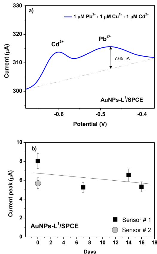
Fig. 12 (a) Selectivity test of the various HMI ions (Pb 2+ , Cu 2+ , and Cd 2+ ) at 1 µM in seawater and (b) reproducibility test of two AuNPs-L¹/SPCE sensors and signal stability test up to 16 days.
