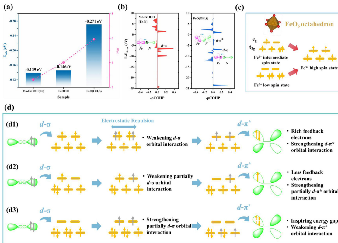
Fig. 6 (a) Spin states and \text{N}_2 adsorption energies of Fe sites for different FeOOH-based catalysts; (b) the -\text{pCOHP} of Fe–N interactions and the electron donation-acceptance process between Fe sites and \text{N}_2 for FeO(OH, S) and Mo–FeOOH; (c) spin states and corresponding d-orbital electronic structures of Fe sites; (d) the possible mechanisms of the spin state effect for the \text{N}_2 activation process.
