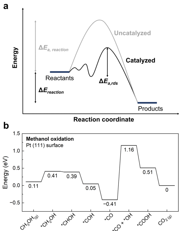
Fig. 6 Energetics of catalysis. (a) Role of catalysts in altering the energetic landscape of the reaction. The uncatalyzed reaction (grey) has a higher activation energy \Delta E_{\text{a}} compared to the catalyzed reaction (black). The reaction energy \Delta E_{\text{reaction}} does not change. \Delta E_{\text{a, rds}} corresponds to the activation energy for the rate determining step in the catalyzed reaction. (b) Reaction energetics profile for MOR on Pt(111) following the indirect pathway. The CO oxidation steps typically are rate-limiting on Pt-based surfaces, as indicated by having the highest thermodynamic reaction barrier. Adapted with permission from ref. 44. Copyright 2012 American Chemical Society.
