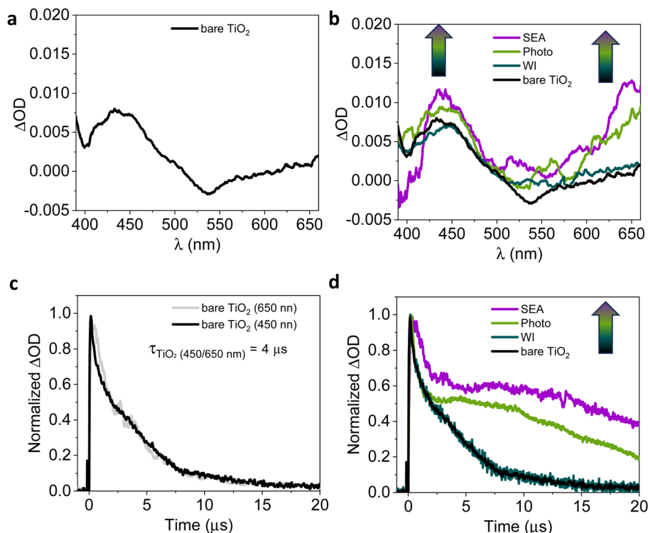
Fig. 5 (a) Transient absorption spectra (TAS, \lambda_{\text{exc}} = 355 nm, 300 mJ) of bare \text{TiO}_2 under Ar. (b) TAS ( \lambda_{\text{exc}} = 355 nm, 300 mJ) of \text{Pd/TiO}_2 (WI), \text{Pd/TiO}_2 (Photo) and \text{Pd/TiO}_2 (SEA) under Ar. (c) Normalised decay traces ( \lambda_{\text{exc}} = 355 nm, \lambda_{\text{mon}} = 450 or 650 nm, 300 mJ) for bare \text{TiO}_2 under Ar. (d) Normalised decay traces ( \lambda_{\text{exc}} = 355 nm, \lambda_{\text{mon}} = 450 nm, 300 mJ) for \text{Pd/TiO}_2 (WI), \text{Pd/TiO}_2 (Photo) and \text{Pd/TiO}_2 (SEA) under Ar. Bare \text{TiO}_2 is included for comparison.
