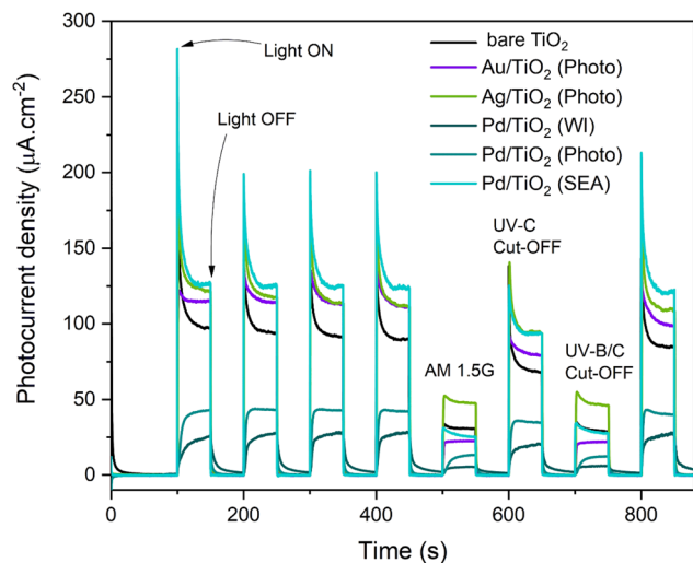
Fig. 3 Chronoamperometric measurements of all synthesised samples and bare \text{TiO}_2 . Signals were recorded in 0.5 M \text{Na}_2\text{SO}_4 , at 0.2 V against Ag/AgCl as the reference electrode; the light was switched ON and OFF every 50 s.
