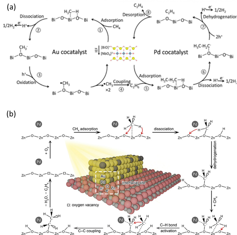
Fig. 14 Schematic representation of photocatalytic NOCM to \text{C}_2\text{H}_4 reaction mechanisms over (a) Au-Pd/ \text{BiNbO}_5\text{F}_6 ; Reproduced with permission. 76 Copyright 2023, American Chemical Society. (b) AuPd/ \text{ZnO} . Reproduced with permission. 73 Copyright 2020, American Chemical Society.
