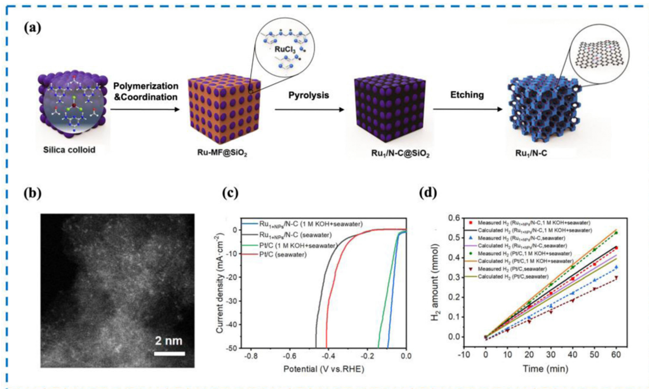
Fig. 10 Synthesis, HAADF-STEM and HER performance of \text{Ru}_{1+n}\text{Ps}/\text{N}-\text{C} . (a) Synthesis of \text{Ru}_{1+n}\text{Ps}/\text{N}-\text{C} . (b) HAADF-STEM image. (c) LSV curve in seawater and 1 M KOH. (d) FE in seawater and 1 M KOH. 188 This figure has been adapted/reproduced from ref. 188 with permission from American Chemical Society, copyright©2022, American Chemical Society.
