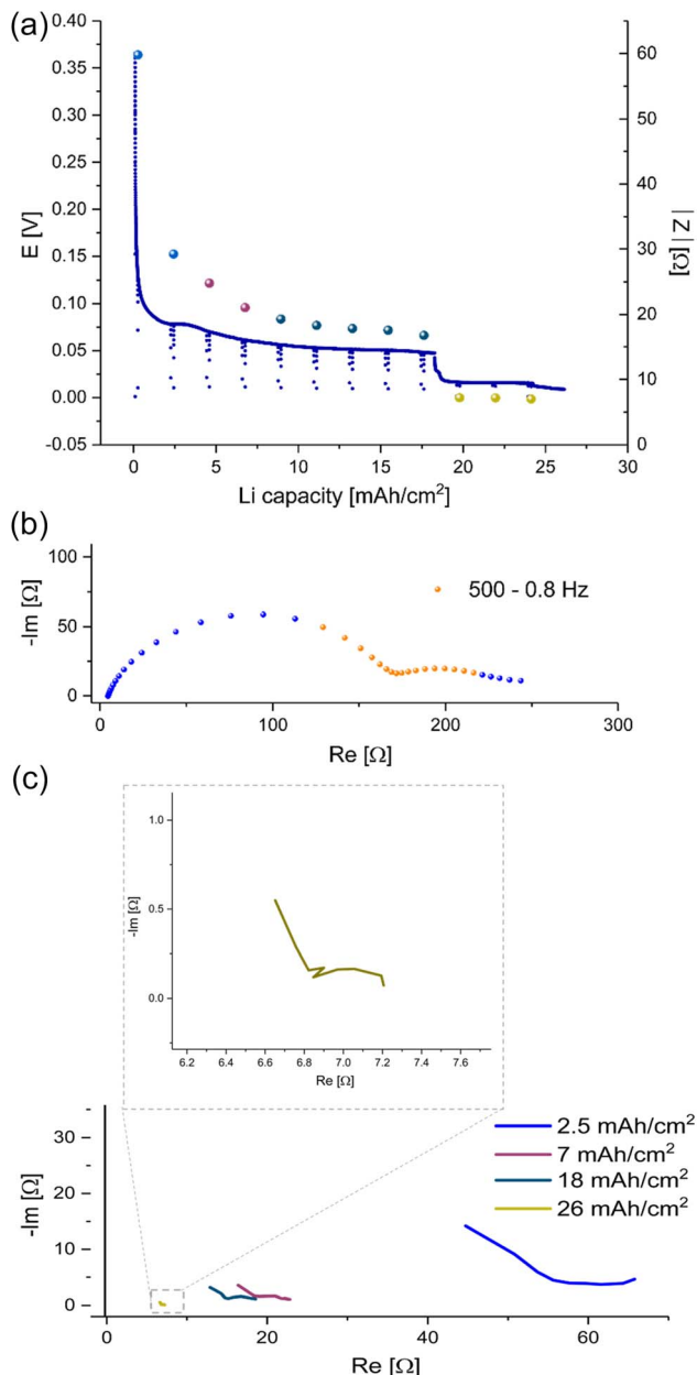
Fig. 4 (a) The voltage trace ( E-t ) of galvanostatic plating a total of 26 mA h cm^{-2} Li at 1 mA cm^{-2} in Li symmetric cell with LP30 electrolyte and GF separator at RT. EIS module values (spheres) were measured with GEIS at 9 Hz with 100 \mu A amplitude at 500–0.8 Hz. (b) A Nyquist plot of the PEIS spectrum of a symmetric lithium cell, LP30 electrolyte with GF separator measured after native SEI formation and before Li plating with 10 mV amplitude at RT. The frequency range used in the following GEIS measurements is indicated in orange. (c) Nyquist plots measured with GEIS, 100 \mu A amplitude at RT during Li plating in a symmetric cell, LP30 electrolyte RT with GF separator. Magnification of the plot measured after plating 26 mA h cm^{-2} Li.
