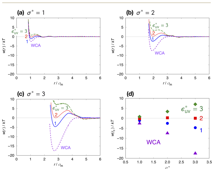
Fig. 2 Effects of the solute–solvent attractive interaction on w(r) for LJ solutes in water at 1 bar and 300 K. The solute diameter is fixed at (a) \sigma^* = 1 , (b) \sigma^* = 2 , and (c) \sigma^* = 3 . Dashed “WCA” curves mark the repulsive WCA potential, and solid, dotted and long dashed curves are the w(r) for solutes interacting with water via the LJ potential with \epsilon_{uv}^* = 1, 2, and 3 , respectively. (d) The first minimum w(r_c) of w(r) as a function of \sigma^* for the four different solute–solvent pair potentials.
