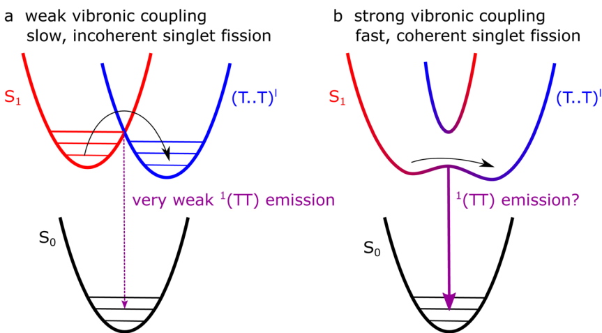
Fig. 13 Possible singlet-fission pathways in crystalline rubrene. (a) In bulk crystals, low energy modes provide weak vibronic coupling between S_1 and triplet pairs (here denoted as (\text{T}..\text{T})^1 ) as in the absence of vibronic/electronic coupling, the triplet pairs are weakly exchange-coupled and mixed-spin states. As a result, singlet fission is incoherent and slow (picosecond timescale). (b) At sites where the symmetry is broken by static disorder, S_1 and triplet pairs can become strongly mixed, allowing fast (femtosecond) coherent formation of ^1(\text{TT}) . We might expect the strength of any Herzberg–Teller emission from ^1(\text{TT}) to follow the strength of vibronic coupling (purple arrows).
