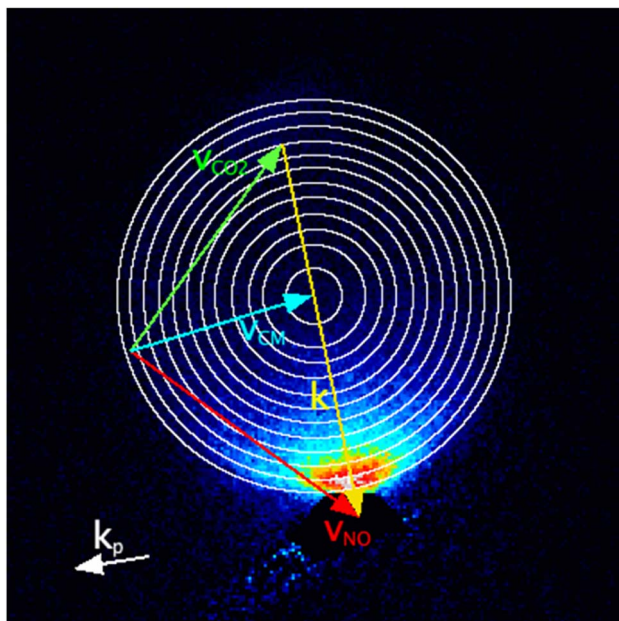
Fig. 1 Newton diagram superimposed on an experimental image for final state N' = 10 . Labels indicate the average laboratory frame velocities of NO ( v_{\text{NO}} ), CO 2 ( v_{\text{CO}_2} ), relative collision velocity ( k ) and the velocity of the centre of mass ( v_{\text{CM}} ). The rings indicate the in-plane scattered final speeds for the 12 values of \Delta E_{\text{CO}_2} . Also indicated is the propagation direction of the probe laser, k_p . NO beamspot-subtraction artefacts have been masked.
