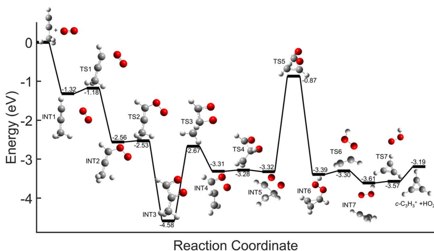
Fig. 7 Global potential energy surface of complex formation leading to \text{c-C}_3\text{H}_3^+ production for \text{O}_2^+ with propyne ( \text{H}_3\text{C}_3\text{H} ) calculated at the \omega\text{b97x/aug-cc-pvtz} level. All energies are displayed relative to reactant energy at infinite separation. Note that states INT1–INT4 are identical to those shown in Fig. 8. These surfaces have been separated for clarity.
