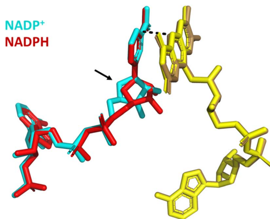
Fig. 10 Structural alignment of Y354S bound to NADP + (PDB 1QFY 21 ) with Y354S bound to NADPH (PDB 1QFZ 21 ); FAD (yellow shades); NADP + (cyan); NADPH (red).
