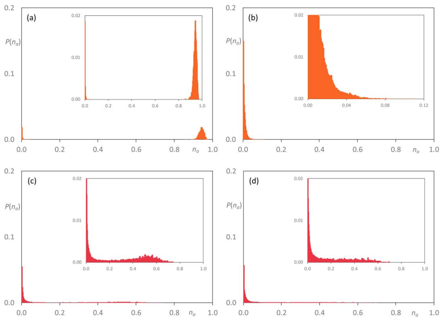
Fig. 13 Discrete probability distribution function, P(n_a) , for [C_{10MIM}]_{1-x}[C_8MIM-F13]_x[Tf_2N] : [C_{10MIM}] chains at (a) x = 0.35 ; (c) x = 0.5 ; [C_8MIM-F13] chains at (b) x = 0.35 ; (d) x = 0.5 .
