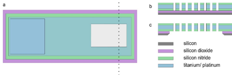
Fig. 2 Schematic showing the (a) common top-down view, demonstrating the exposed contact pad (blue, left) and array (grey, right) area, and the cross-sectional views of (b) the MNEE array and (c) MNE array areas (not to scale, number of elements in array is illustrative only).
