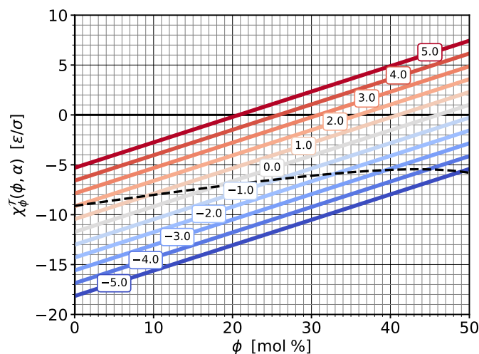
Fig. 8 Susceptibility \chi_{\phi|\alpha}^{\mathcal{T}} from Eqn. (13d) as a function of cholesterol content \phi , parametrized by different values of phospholipid abundance \alpha , as indicated in the boxed labels, and the saturation ratios from Eqns (18). The dashed line shows the susceptibility for the special \phi -dependent \alpha value at which \mathcal{T} = 0 (i.e., on the zero-torque contour in Fig. 7).
