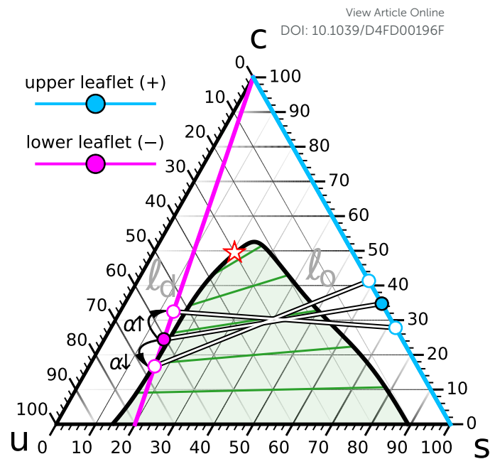
Fig. 11 The set of saturation ratios r_+ = 1 for leaf + (cyan line) and r_- = 0.2 for leaf - (magenta line), combined with an overall cholesterol content \phi = 30\% , yields a pair of coexisting points (solid cyan and magenta symbols) of which the leaf - composition resides very close to the \ell_d -side of the binodal. Increasing the abundance asymmetry \alpha \rightarrow +10\% squeezes cholesterol from leaf + to leaf - and pushes the latter further away from the two phase region. Reducing \alpha \rightarrow -10\% instead removes cholesterol from leaf - and plunges it into \ell_o/\ell_d coexistence (see Fig. 12 for illustrations). The compositions in leaf + pivot oppositely but always stay in a homogeneous \ell_o phase.
