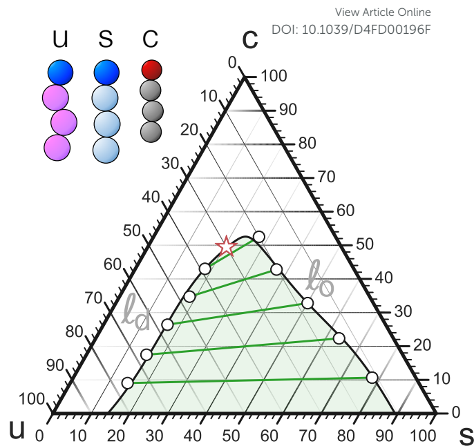
Fig. 6 Phase diagram of a ternary mixture in the Cooke lipid model of a lipid mixture, showing l_o/l_d coexistence and (the approximate location of) its critical point (adapted from Ref. [ 98]).
