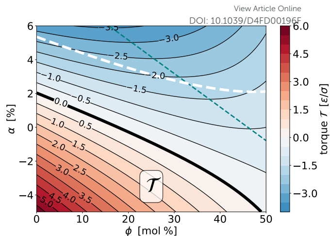
Fig. 7 Contour plot of the (empirically fitted) torque surface \mathcal{T}(\phi, \alpha) for the saturation ratios r_- = 0.125 and r_+ = 0.833 . The bold solid curve is the location where the torque vanishes and hence GUVs would be mechanically stable, the thin teal dashed curve is the nullcline at which \partial \mathcal{T} / \partial \phi = \chi_{\phi|\alpha}^{\mathcal{T}} = 0 , i.e. , where the torque does not change upon small variations of overall cholesterol content. The bold white dashed curve is the locus of states for which \Delta \Sigma = 0 (see also Fig. 10).
