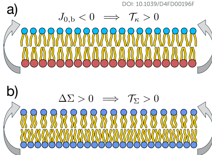
Fig. 2 Clarifying the sign of the torque, \mathcal{T} = \mathcal{T}_\kappa + \mathcal{T}_\Sigma . a) The torque due to lipid curvature, \mathcal{T}_\kappa , strives to bend the membrane up when the spontaneous bilayer curvature is negative, J_{0,b} < 0 , i.e. when the upper leaflet has a more negative spontaneous curvature than the lower one. b) The torque due to differential stress, \mathcal{T}_\Sigma , strives to bend the membrane up when the differential stress is positive, \Delta\Sigma > 0 , i.e. when the upper leaflet is under excess tension.
