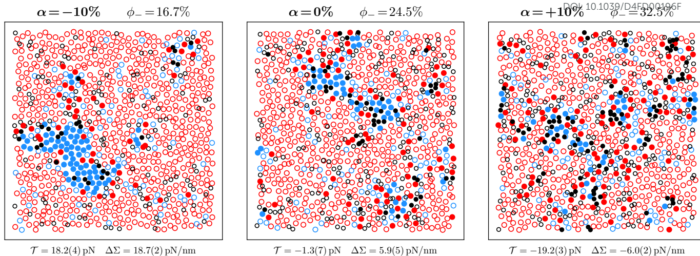
Fig. 12 Stylized representative lipid configurations in leaf - of the three systems discussed in Sec. 4.3 and represented in the phase diagram of Fig. 11. Colors indicate lipid type—red: unsaturated, blue: saturated, black: cholesterol—while style indicates the phase state—open circles: l_d , filled circles: l_o —as identified by a Hidden Markov Model analysis. 98,109 At zero abundance, the phase state in leaf - is very close to the l_d -side of the coexistence binodal and we see only fleeting occurrences of small transient l_o regions. At \alpha = -10\% cholesterol is drawn out of leaf - which pushes the phase state into the coexistence region and we get a small but persistent l_o domain. Conversely, at \alpha = +10\% cholesterol is pushed from leaf + into leaf - , increasing the state's distance from the coexistence region and further melting any remaining ordered domains. All systems contain 2048 lipids, and the box length is approximately L \approx 32 \sigma \approx 24 \text{ nm} .
