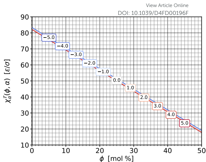
Fig. 9 Susceptibility \chi_{\alpha|\phi}^{\mathcal{T}} from Eqn. (13b) as a function of cholesterol content \phi , parametrized by different values of phospholipid abundance \alpha , as indicated in the boxed labels. The lines almost coincide, with smaller \alpha values having ever so slightly larger susceptibilities.
