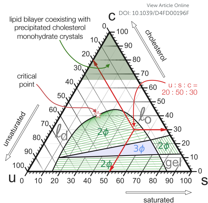
Fig. 1 Gibbs triangle representation of a typical ternary phase diagram of a lipid mixture of saturated , unsaturated , and cholesterol lipids. This image is merely a schematic, but it qualitatively reflects the basic topography measured in many experimental studies. White regions correspond to pure phases, hatched green regions exhibit two-phase coexistence, with the green lines actually being the tie-lines between coexisting phase points. The central blue triangle is a region of three-phase coexistence, in which the pure phases at the triangle’s corners coexist. The three red arrows illustrate how to read off the composition of some given point. The sum of their lengths is the same no matter which point in the triangle we pick, which is the key geometric fact that enables this representation in the first place.
