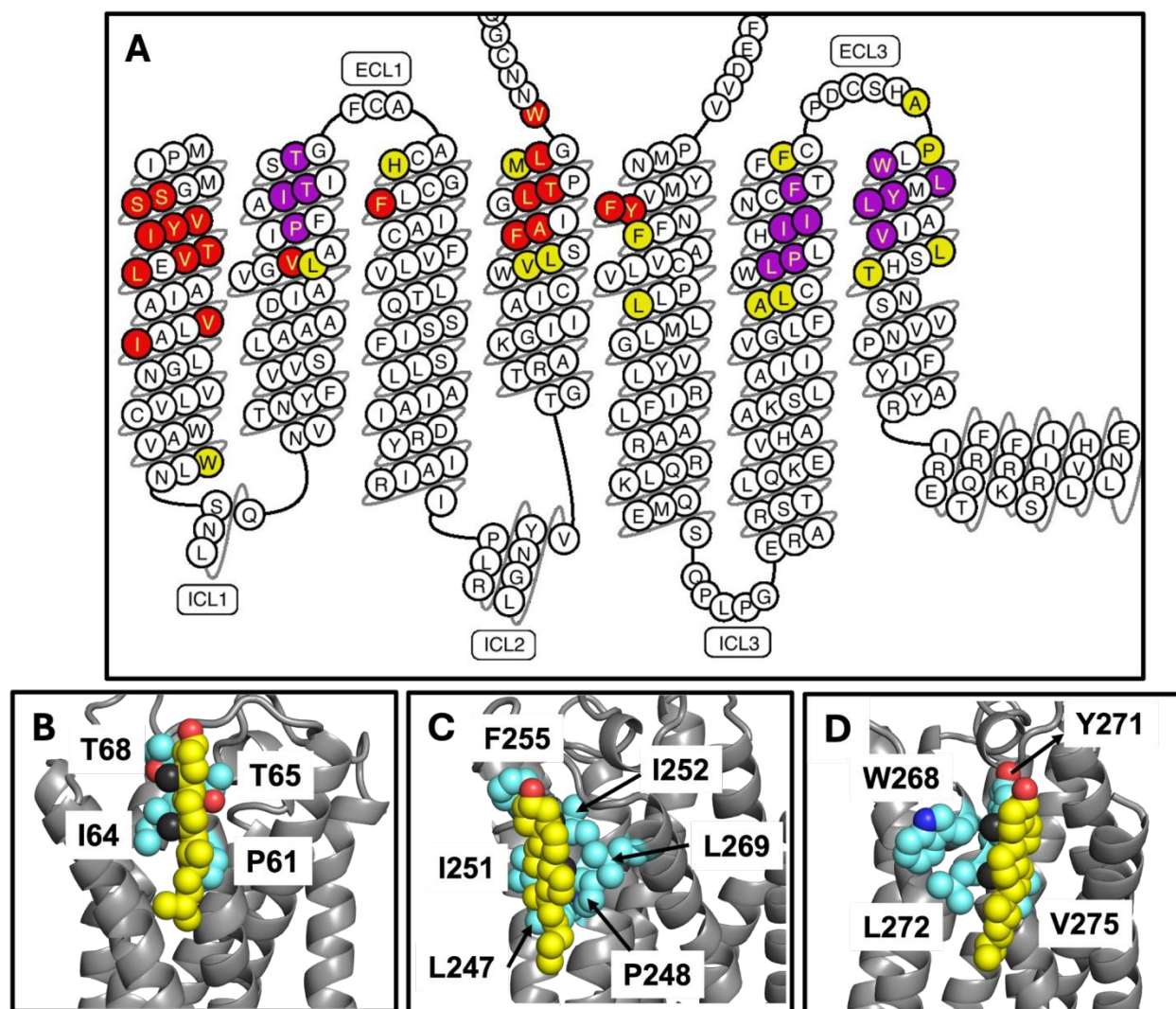
Figure 4 Cholesterol interactions with the receptor in the asymmetric membrane simulation. Interactions are colored by residue in panel A, with purple indicating interaction with a single cholesterol for the entire duration of the simulation, red indicating interaction with any cholesterol for at least 80% of the simulation, and yellow any cholesterol for at least 50% of the simulation. The binding disposition of the cholesterol on helix 2 is shown in panel B, on helix 6 in panel C, and on helix 7 in panel D. The heavy atoms of the sidechains indicated in purple in panel A are represented with cyan spheres and are labeled in panels B-D. Carbon atoms in cholesterol are yellow spheres, the red sphere shows the hydroxyl oxygen, and the black spheres represent the methyls of the beta face. The same analysis is shown for the symmetrized membrane simulation in Supplemental Figure S6 .
