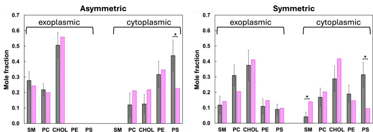
Figure 2 The mole fraction of lipids in each class in the first solvation shell in the exoplasmic and cytoplasmic leaflets, and in the asymmetric membrane simulation (left panel) and in the symmetric membrane simulation (right panel), averaged over the last 5 \mu sec simulations. Gray filled bars are the results for the first solvation shell of the receptor, and the magenta filled bars
