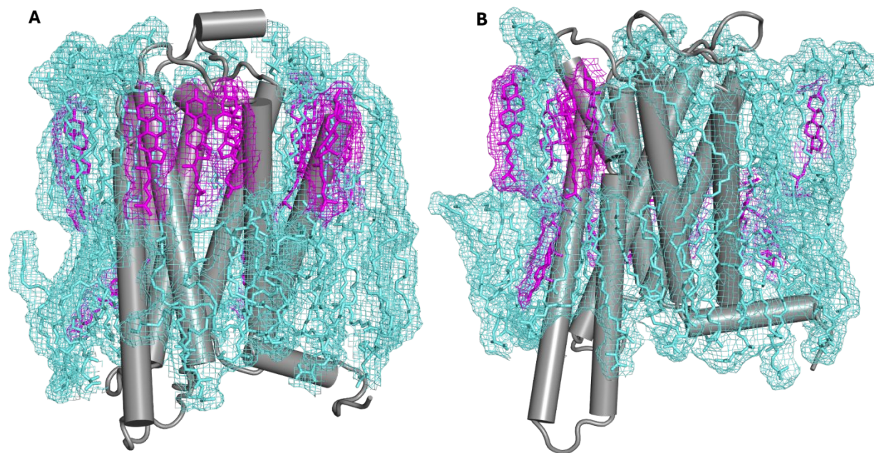
Fig. 1 Simulation snapshot showing the A 2A adenosine receptor in an asymmetric plasma membrane model (panel A) and its symmetrized counterpart (panel B). First shell cholesterols are rendered in pink and other first shell lipids in cyan. Wireframe mesh shows the outline of the lipid mass density. Each snapshot is the final configuration of a 10 \mu sec all-atom simulation.
