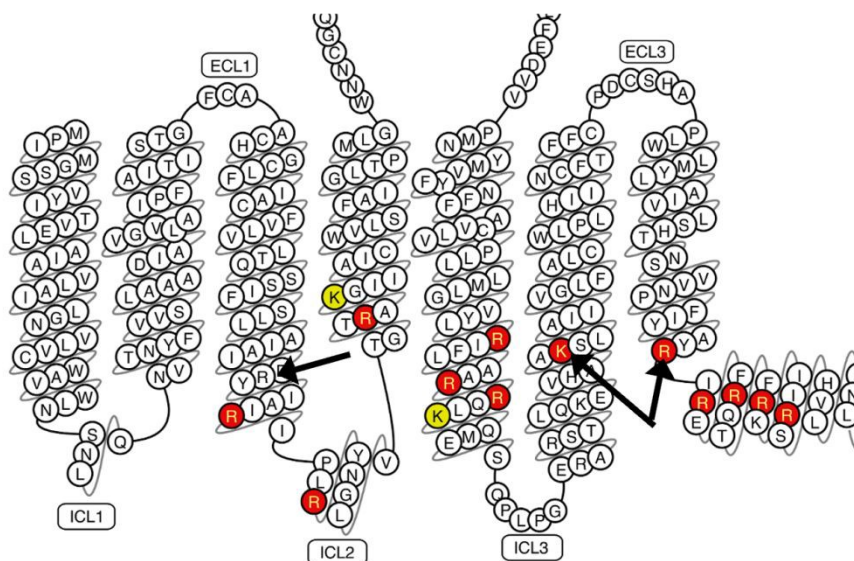
Figure 3 Positively charged side chains that interact with a PS headgroup at least 80% of the time in the asymmetric membrane simulation (red) or at least 50% of the time (yellow). The arginine of the D/ERY motif is marked on helix 3 with a black arrow. K233 6,35 and R291 7,56 mediate a PS interaction motif that allosterically activates the receptor; these are indicated by black arrows on helices 6 and 7. For the corresponding plot from the symmetric membrane simulation, see Supplemental Figure S3 .
