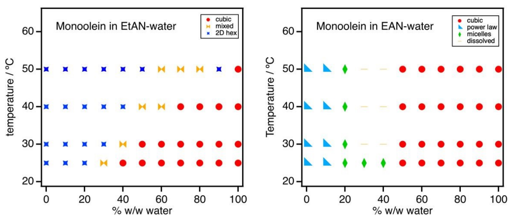
Figure 2: Phases formed by 5% w/w monoolein in (left) EtAN- and (right) EAN- water mixtures. Schematic isothermal ternary phase diagrams drawn combining our data with available literature are shown in Figure S11.
