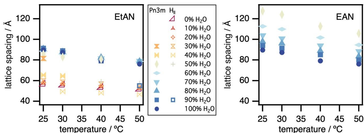
Figure 3: Lattice spacings for the swollen Pn3m cubic and H_{II} phases for monoolein in excess EtAN-water and EAN-water mixtures. The error bars are smaller than the marker sizes.
