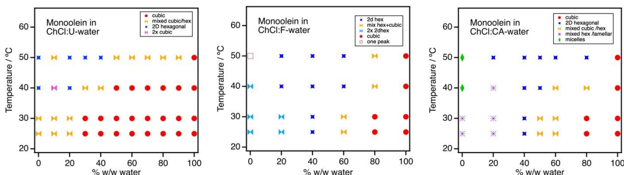
Figure 6: Phases observed in 5% w/w monoolein in ChCl:U-water, ChCl:F-water and ChCl:CA-water mixtures. Schematic isothermal ternary phase diagrams are shown in Figure S13.
