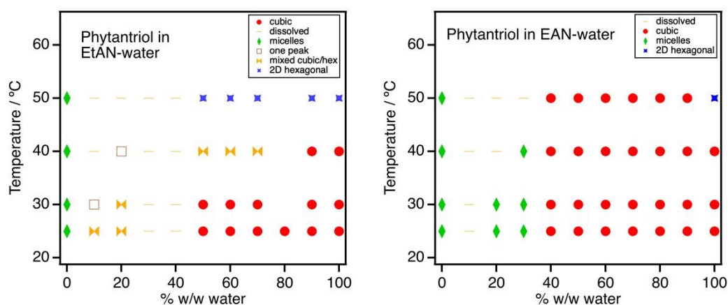
Figure 4: Phases formed by 5% w/w phytantriol in EtAN-water (left) and EAN-water (right) mixtures. Schematic isothermal ternary phase diagrams are shown in Figure S12.
