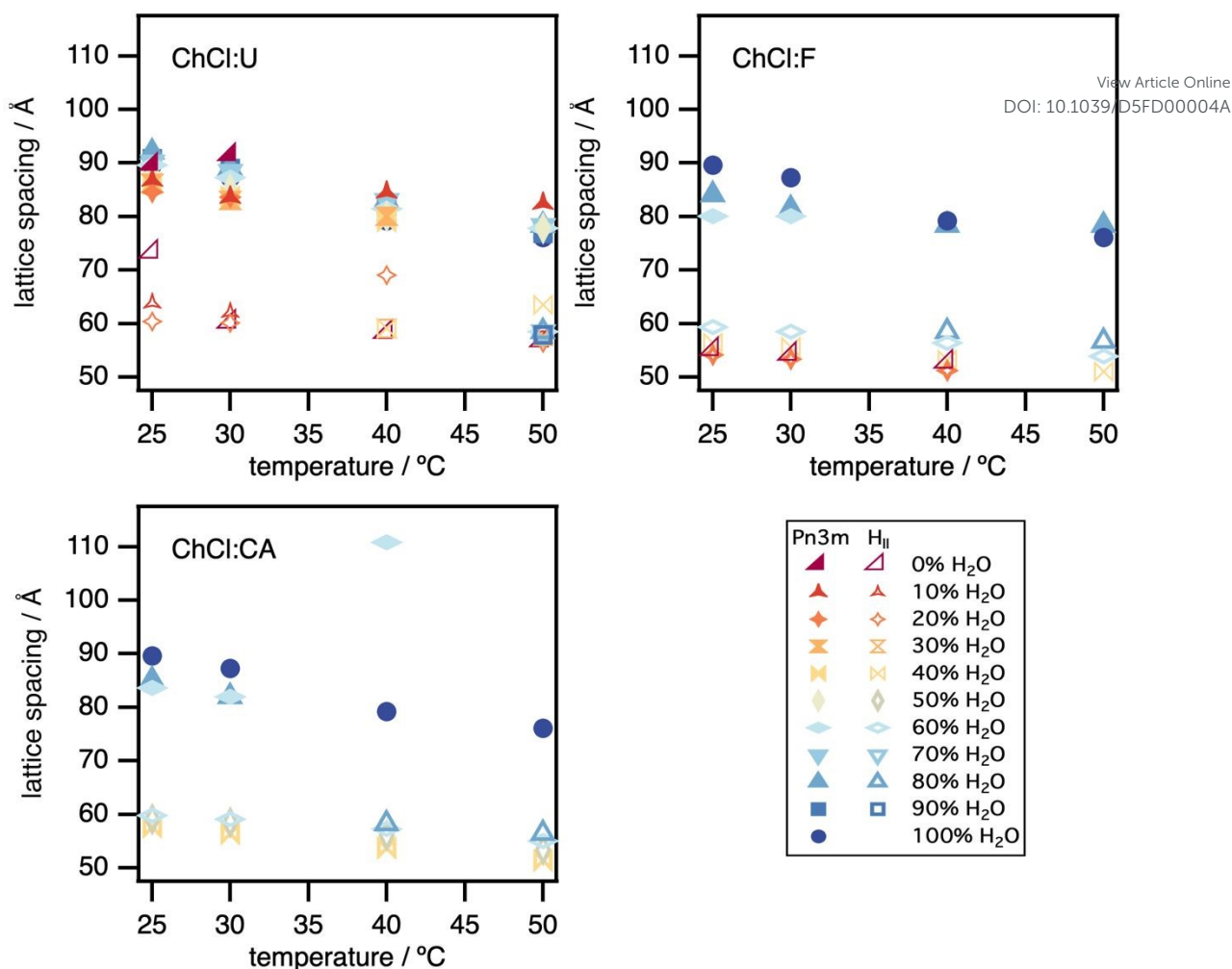
Figure 7: Lattice spacings for the Pn3m cubic and H_{II} phases observed for monoolein in ChCl:U -water, ChCl:F -water and ChCl:CA -water mixtures. The error bars are smaller than the marker sizes. Where two H_{II} phases are observed, the larger lattice spacing is plotted.
