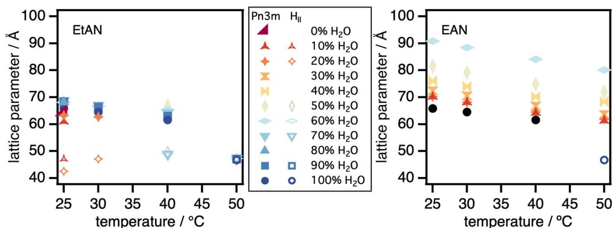
Figure 5: Lattice parameters of the Pn3m cubic and H II phases observed for phytantriol in EtAN-water and EAN-water mixtures. The error bars are smaller than the marker sizes.
