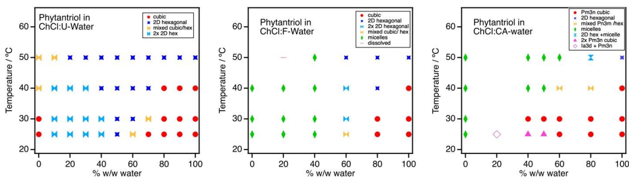
Figure 8: Phases observed for phytantriol in ChCl:U -water, ChCl:F -water and ChCl:CA -water mixtures. Schematic isothermal ternary phase diagrams are shown in Figure S14.
