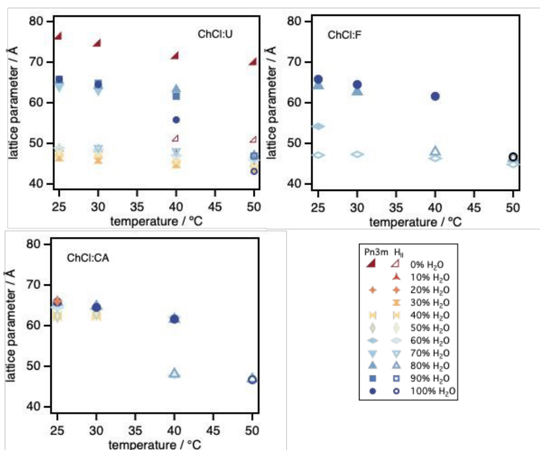
Figure 9: Lattice spacings for the Pn3m cubic and H II phases observed for phytantriol in ChCl:U-water, ChCl:F-water and ChCl:CA-water mixtures. The error bars are smaller than the marker sizes.
