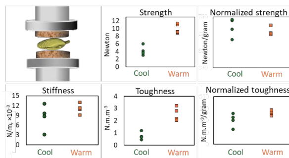
Figure 4. Micromechanical testing of 4 complete shells per group in compression. Strength and toughness are presented as absolute values and normalized by the shell weight. Stiffness is shown only as absolute values. The shells were selected to be approximately of the same size of ~4-5 mm. Cool-water shells weight varied between 0.006-0.009 g; warm-water shells weight varied between 0.018-0.022 g.
