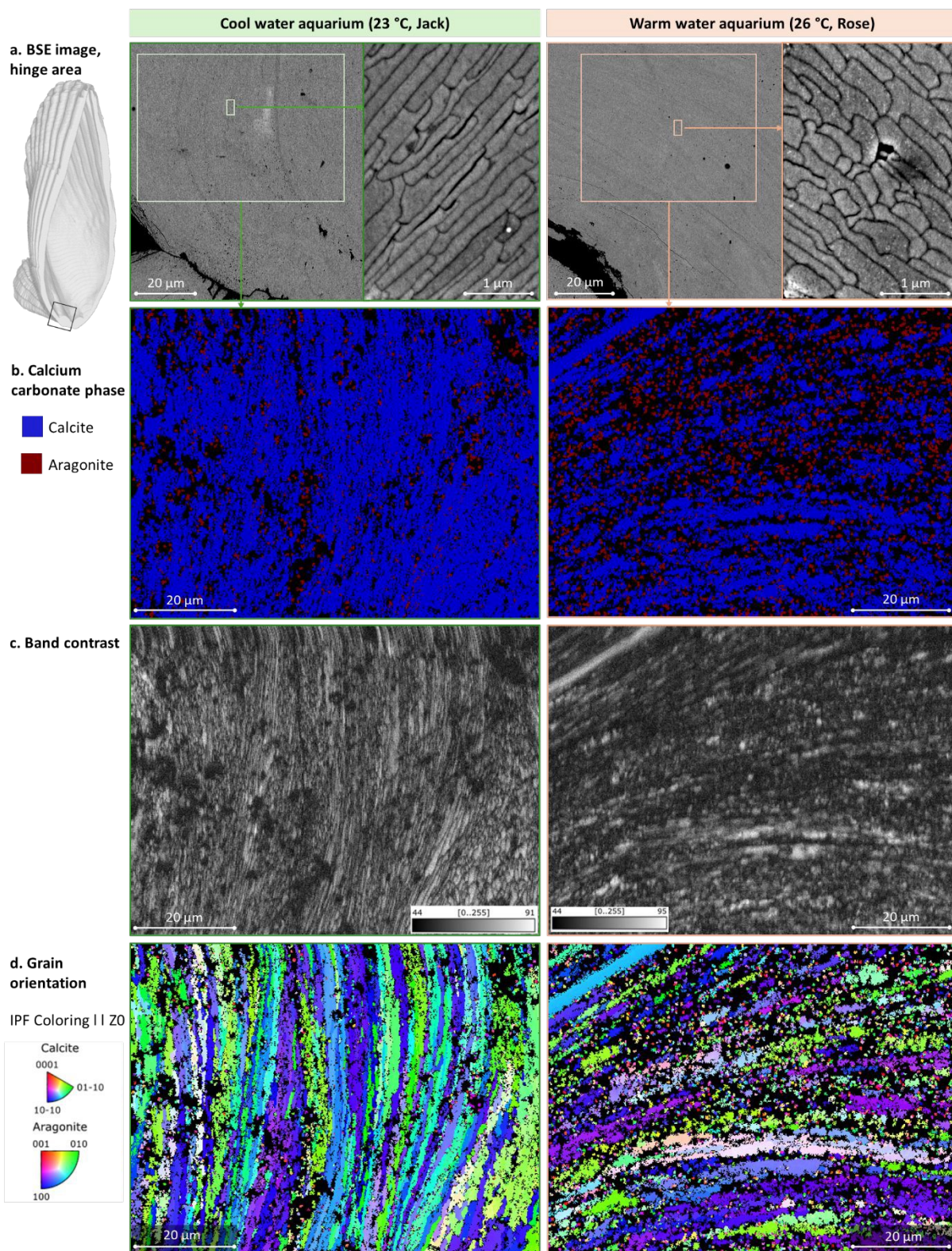
Figure 6. Microstructure and crystallographic analysis near the hinge of the shell cross-section of scallops grown in cool (left panel) and warm (right panel) water. (a) Backscattered electron (BSE) images of the shell cross-section. Insets show the BSE images at higher magnification of the area
