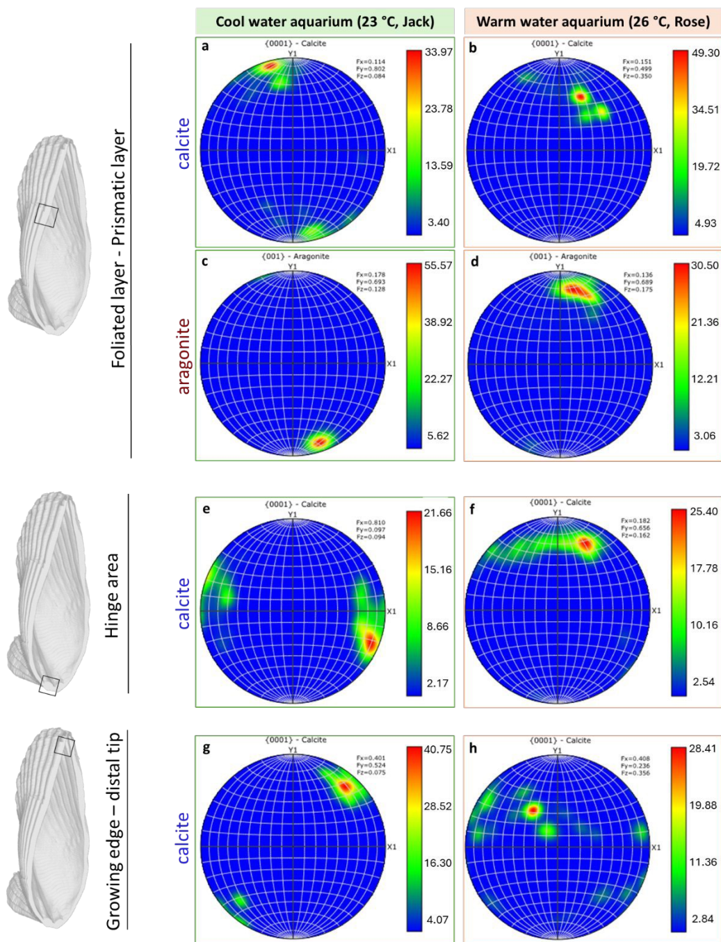
Figure 8. Pole figures for calcite and aragonite representing the entire orientation maps shown in Figure 5 (a-d), Figure 6 (e,f) and Figure 7 (g,h). Scale is given in multiples of uniform distribution (MUD).
