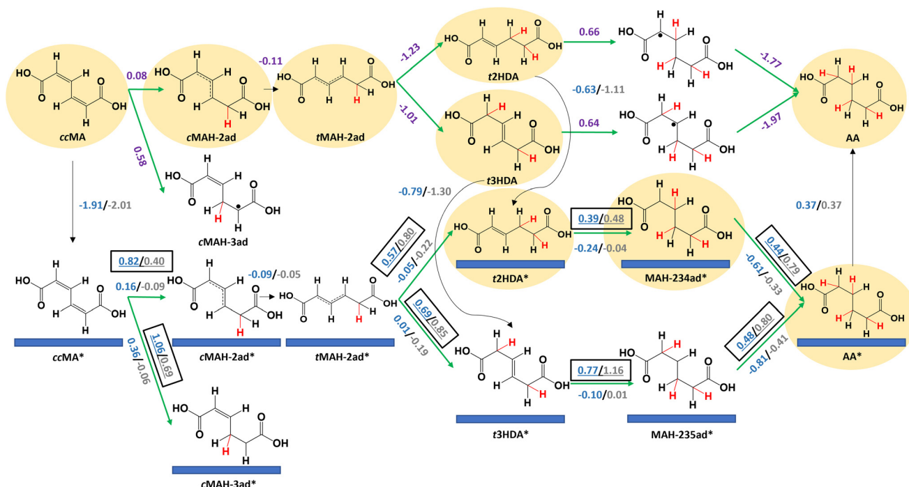
Fig. 3 Reaction energetics at -0.14 V_{RHE} and 298 K for elementary steps in electrochemical hydrogenation of cis,cis -muconic acid ( ccMA ) to trans -2-hexenedioic acid ( t2HDA ), trans -3-hexenedioic acid ( t3HDA ), and adipic acid ( AA ) on Pd(111) [blue], Pt(111) [grey], and in solution [purple]. Green arrows denote electrochemical steps and black arrows denote non-electrochemical steps. Activation free energies ( G_a , eV) are underlined and boxed; reaction free energies ( \Delta G , eV) are also provided (not underlined or boxed). The H atoms added to ccMA during ECH are highlighted in red for clarity. "*" denotes adsorbed species. "." denotes an unpaired electron. The species involved in the energetically preferred pathway are highlighted.
