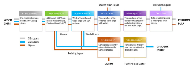
Fig. 7 The Fabiola process (reproduced from ref. 79 with permission from the authors. Published by American Chemical Society, copyright 2022).
