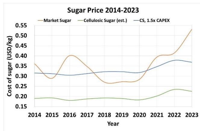
Figure 4. Comparison of sugar prices for glucose derived from corn stover and US trading price for sugar from 2014-2023. US sugar (brown) price data taken from the US Federal Reserve Economic Data database. 49 Cellulosic sugar price adapted from the techno-economic model for ionoSolv corn stover 14 corrected for CEPCI cost factors and energy prices (green) and also with a 1.5x CAPEX increase to reflect uncertainty in new technology prices (blue).
