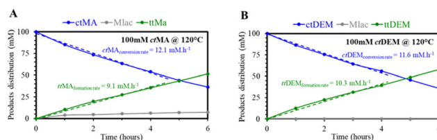
Fig. 6 The time profile of the isomerization of 100 mM ctMA and ctDEM in DMSO (5 mL) and 2eq. \text{H}_2\text{O} at 120 °C. The rate plots for the conversion of ct -isomer and the formation of the tt -isomer are obtained for the slope of the data points plotted between 0 and 4 hours. The reactions were performed in glass pressure tubes sealed under static conditions. The product distribution was determined by ^1\text{H} -NMR for the reaction in A and by GC for the reaction in B.
