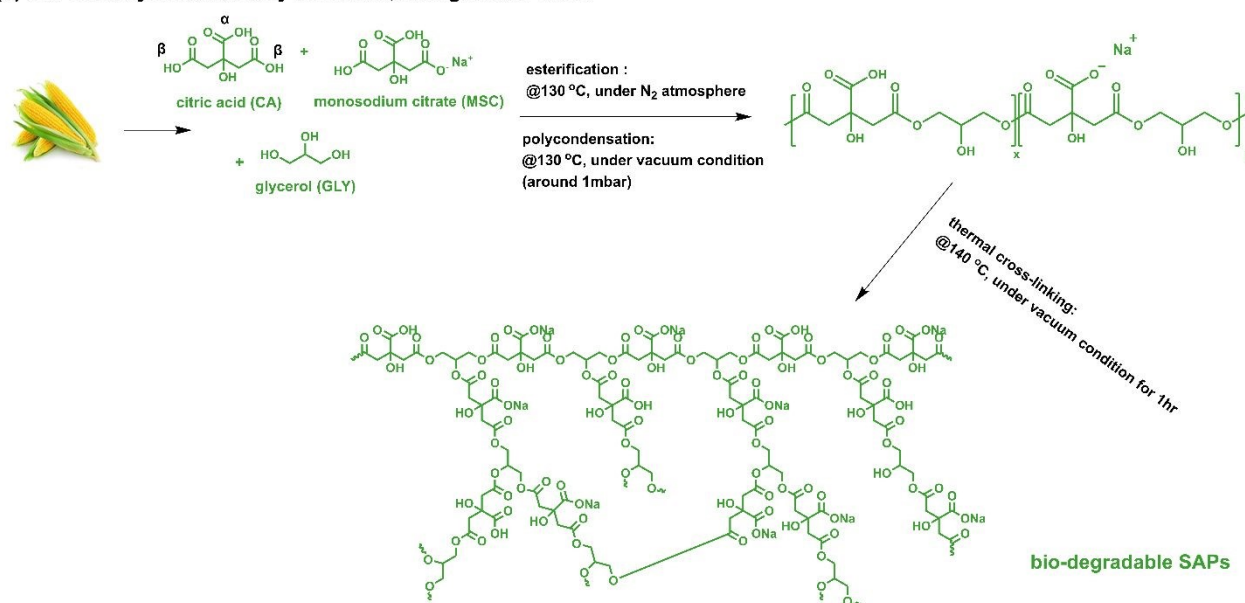
Scheme 1. Comparison between Synthesis of CA+MSC/GLY-based SAP and conventional SAP. x denotes the molar percentage of citric acid in the total moles of acid (CA + MSC) in the feed
