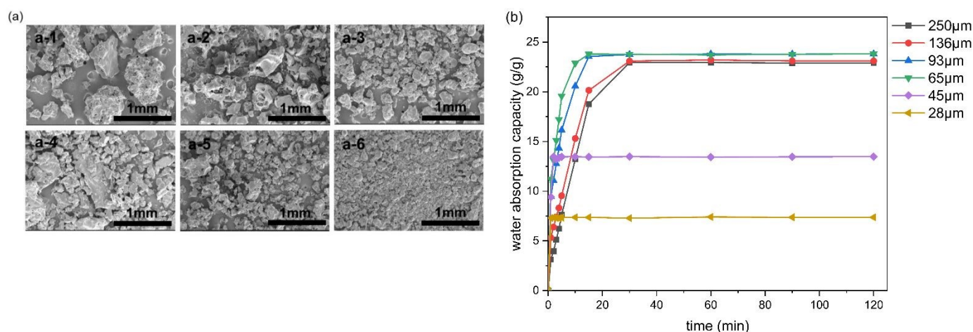
Figure 3. (a) SEM images of cross-linked (at 140 °C) and extracted SAP-80 particles ground for different times (30, 60, 120, 150, 180, 210 s, respectively); (b) Plot of water absorption capacity versus swelling time (samples: cross-linked (at 140 °C) and extracted SAP-80, ground to D_{circle\ equivalent} values of 250, 136, 93, 65, 45 and 28 \mu\text{m} obtained after grinding times varying from 30 to 210 s, respectively).
