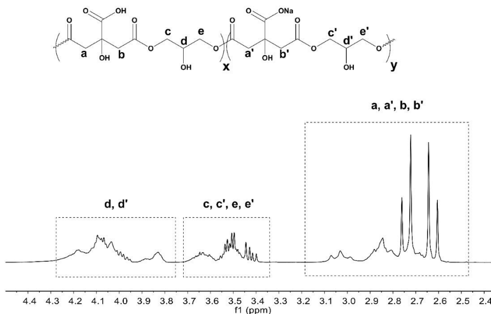
Figure 1. NMR spectrum of PGC 70 M 30 SAP precursor polymer (All peaks were assigned according to literature reported by Mattoso et al [24].)
