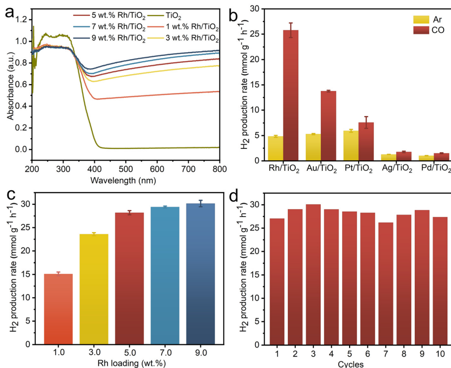
Fig. 3 (a) Absorption spectra for \text{TiO}_2 and x wt% \text{Rh}/\text{TiO}_2 ; (b) triphase photocatalytic \text{H}_2 production rate for 5 wt% \text{M}/\text{TiO}_2 ( \text{M} = \text{Rh}, \text{Au}, \text{Ag}, \text{Pt}, \text{Pd} ) in Ar or CO atmosphere; (c) photocatalytic \text{H}_2 production rate as a function of the loading amount of Rh in \text{Rh}/\text{TiO}_2 ; (d) cycling tests for \text{Rh}/\text{TiO}_2 . Reaction conditions: gas phase = 0.2 MPa of CO, liquid phase = 10 mL of \text{H}_2\text{O} , solid phase = 2 mg of photocatalyst immobilized on GDL (4 cm in diameter), light source = 365 nm LED ( 300 \text{ mW cm}^{-2} ). Error bars represent the standard deviation from at least three independent measurements.
