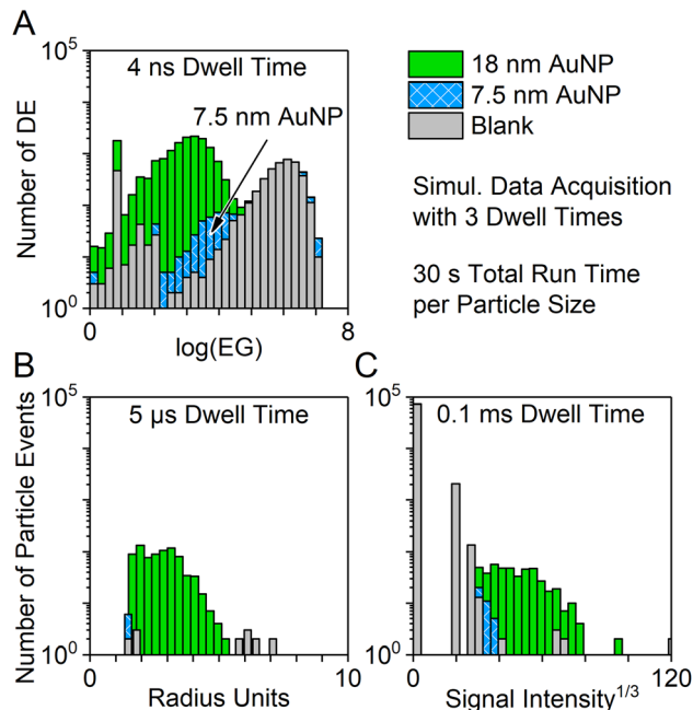
Fig. 8 Comparison of spICP-MS data acquired simultaneously with (A) 4 ns (nanoDAQ), (B) 5 \mu s ( \mu sDAQ), and (C) 0.1 ms (vendor software) dwell time. Dispersions of AuNP with nominal sizes of 18 and 7.5 nm and a blank solution were measured for 30 s, respectively. Please note that the background signal of nanoDAQ data is on the right side (high \log(\text{EG}) ), while the background in plots from conventional spICP-MS is on the left.
