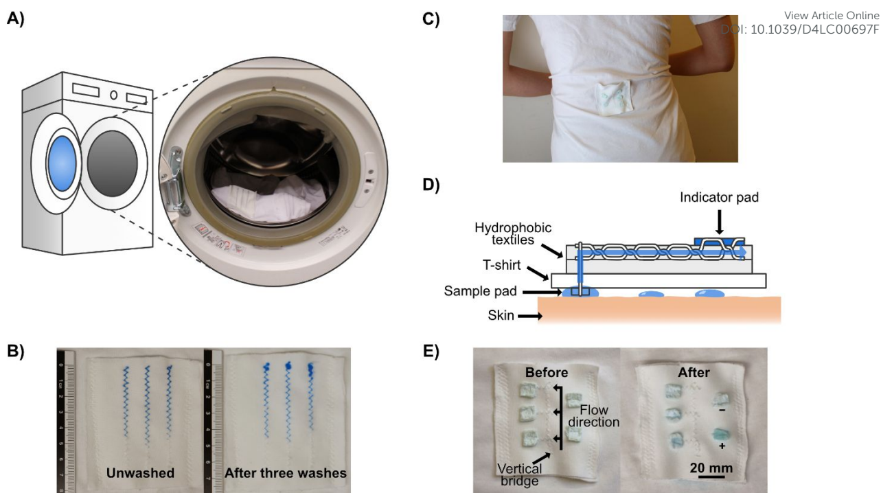
Figure 4: Wearable stitched textile-based microfluidic devices. A) Schematic with an embedded photograph of a T-shirt loaded into a washing machine. The T-shirt had microfluidic devices sewn onto it. B) Comparison of flow behavior in a stitched microfluidic device before the first wash and after three washes. C) Photograph demonstrating wearable stitched textile-based microfluidic devices. The microfluidic device collects and transports sweat to anhydrous copper sulfate moisture indicator pads. The microfluidic device is positioned on the lower back region of the T-shirt. D) Side-on schematic of the wearable textile-based microfluidic sweat analyzing device. E) Comparison of the wearable textile-based microfluidic sweat analysis device before and after sweat collection. The blue color in the first and second indicator pads along the microfluidic channel indicates positive collection. In the after picture, artificial sweat has been added to one of the indicator pads not connected to the microfluidic flow as a positive control.
