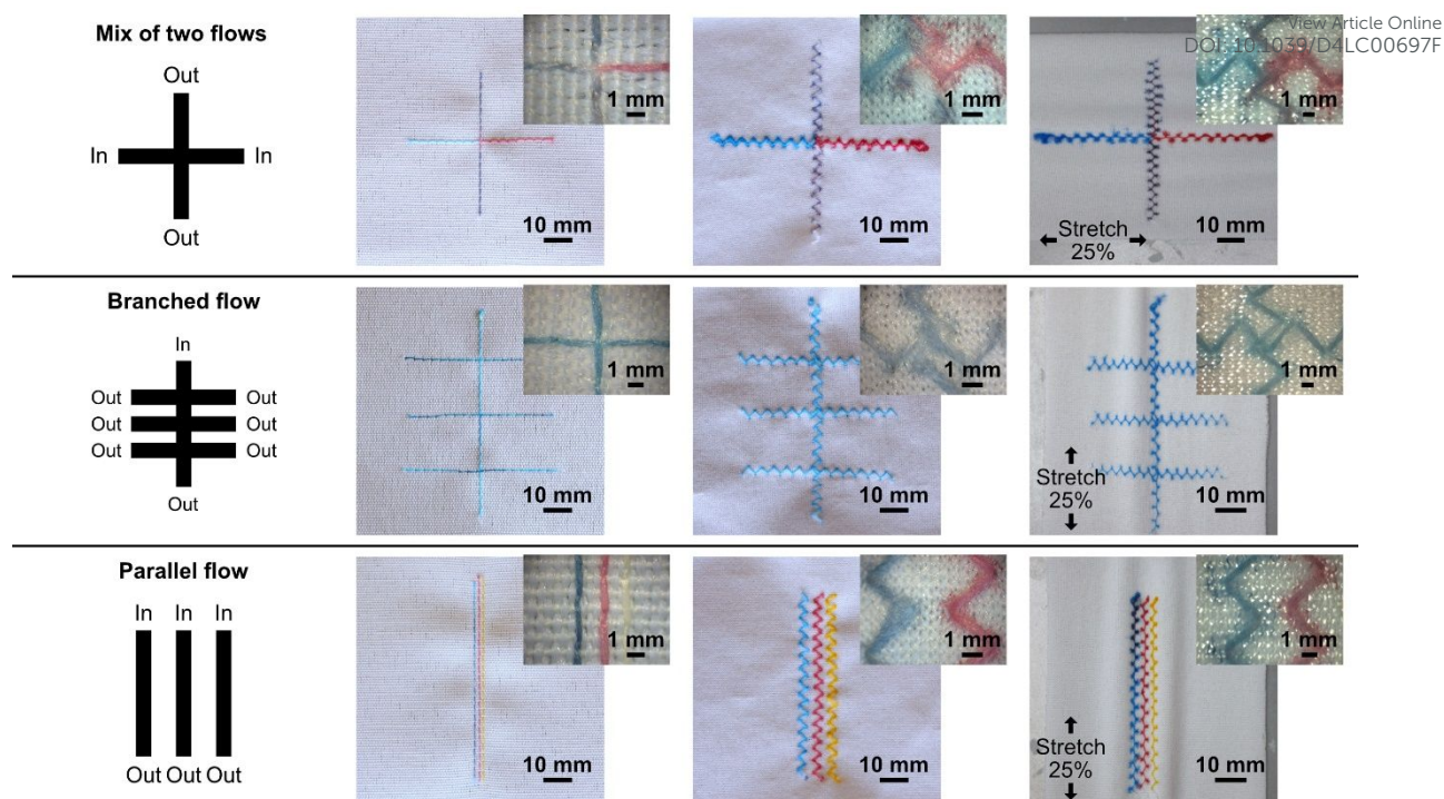
Figure 2: Fundamental microfluidic functions using stitched Coolmax® threads in hydrophobic fabrics. The leftmost column shows a schematic of each function. The three columns to the right show photographs of the corresponding function realized, in order: in woven, knitted, and stretched knitted fabric. The top corners show the corresponding microscope magnification of the stitches.
