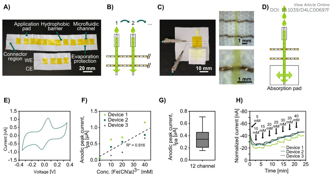
Figure 5: Stitched textile-based electroanalytical microfluidics. A) Photograph of stitched electroanalytical sensing devices with twelve (top) and four (bottom) microfluidic channels with components labeled in the images. B) Schematic of the flow in microfluidic channels across stitched electrodes in the electrofluidic device showing the microfluidic Coolmax ® in white, the Au-coated threads in gold, and the fluid flow in green. C) Photograph of a stitched electroanalytical device capable of continuous monitoring during flow (top side of the device shown in the picture) with embedded microscope images of the intersection between the microfluidic channel and the electrodes. D) Schematic of flow in the electrofluidic device capable of continuous monitoring during flow, showing the microfluidic Coolmax ® in white, the Au-coated threads in gold, and the fluid flow in green. E) An example cyclic voltammogram of 40 mM ferricyanide in the stitched electroanalytical device at a scan rate of 30 mV/s. F) Plot of anodic peak current versus analyte concentration, n = 3 . G) Box plot of anodic peak current from twelve microfluidic channels on the same stitched electroanalytical device. A ferricyanide concentration of 30 mM was used in all channels. H) Normalized chronoamperometric data under the continuous flow solutions with increasing ferricyanide concentrations in three stitched electroanalytical devices.
