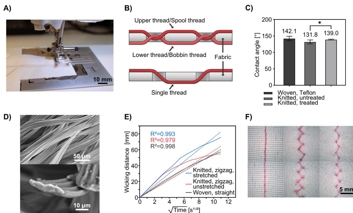
Figure 1. Characterization of fabrics and stitched Coolmax ® threads. A) Photograph showing the fabrication process of stitched textile-based microfluidic devices with a conventional sewing machine. Here the spool and bobbin threads were both Coolmax ® and the machine was prepped to stitch a microfluidic channel across a pair of pre-stitched gold thread electrodes. B) Schematic illustration of a basic lockstitch compared to a hand-sewn stitch. C) Contact angle measurements on the woven fabric and the knitted fabric. The values are averages of three 9 \mu L drops with two replicate measurements on each drop (n=6). Legend: Asterisk (*) means significant difference ( p \leq 0.05 ). D) SEM pictures of the Coolmax ® thread. Top: Side-view. Bottom: Cross-section. E) Wicking behavior of the Coolmax ® thread when stitched in the woven and knitted fabrics. Wicking distance is plotted against the square root of time and fitted to the Washburn equation. F) Magnifications of the sewn stitches in the fabrics. From left to right: Straight interlock stitches in woven fabric, zigzag interlock stitches in knitted fabric (unstretched), zigzag interlock stitches in knitted fabric (stretched). The top row shows the upper thread on the right sides of the fabrics and the bottom row shows the bobbin thread on the wrong sides. The fabrics are oriented with the weft and wale directions horizontally, respectively. Captured with a Dino-Lite RS Pro (AnMo Electronics Corporation, Taiwan).
