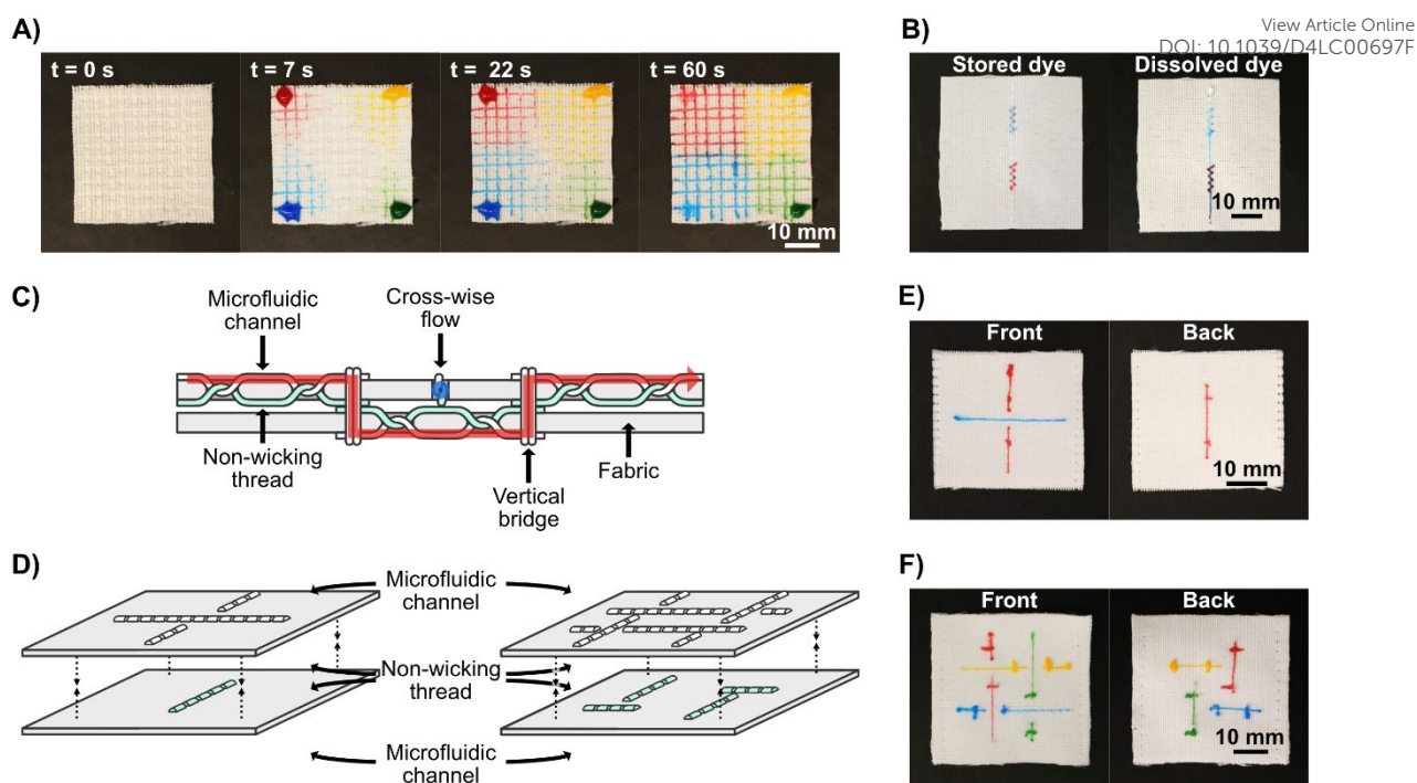
Figure 3: Advanced microfluidic functions in stitched textile-based microfluidic devices. A) Sequential view of liquid flow through a 4 x 4 cm stitched device with 100 microfluidic channel crossings. B) Demonstration of chemical storage in stitched Coolmax ® thread. The zigzag stitches contained dried dye which was rehydrated and transported with the liquid flow after MilliQ water was added to one end of the straight stitch (top of the picture as shown). As the water passes through both storage regions, the colors of the dyes mix. C) Sideview schematic of the 3D stitched microfluidic device. The microfluidic channels of the two layers, aligned through the z-axis, are connected with stitches that pass through both layers vertically. Since there is no fluid path between the perpendicular flows on the top and bottom faces of the device, they do not mix. D) Oblique schematic view of the 3D stitched microfluidic device. Two layers of hydrophobic fabric are stitched with Coolmax ® as the spool thread and non-wicking nylon monofilament as the bobbin thread. The faces of the fabrics with the non-wicking thread are stitched together facing each other. E) Photographs of the two faces of a complete 3D stitched textile-based microfluidic device with a single underpass crossing, showing that the flows of the two different dyes (blue and red) were kept separate. F) Photographs of the two faces of a complete 3D stitched textile-based microfluidic device with four intertangled microfluidic channels, with separated liquid flows.
