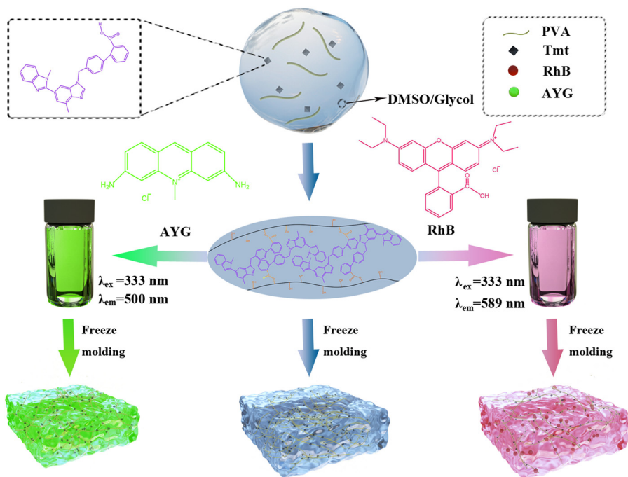
Fig. 1 Schematic of the formation, structure and intermolecular non-covalent interactions of the PVA/Tmt organogel and the prepared light-harvesting systems.
