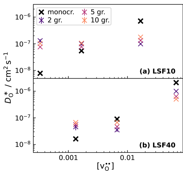
Fig. 13 Oxygen tracer diffusion coefficients in polycrystalline LSF at T = 1800 \text{ K} , extracted from Fig. 11, as a function of [\text{v}_\text{O}] .
