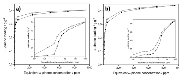
Fig. 1 Gravimetric sorption isotherms of \alpha -pinene recorded at 303\text{ K} on a) DUT-4(Al) and b) MIL-100(Fe) powder, increasing (filled black squares) and decreasing (empty black squares) \alpha -pinene concentration. Insets show the isotherms on a semi-logarithmic basis. Lines are guides for the eyes.
