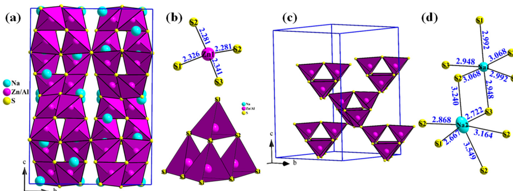
Fig. 3 (a) Projection view of the crystal structure of Na 3 ZnAlS 4 along [100], (b) (Zn/Al) 4 S 4 tetrahedron and (Zn/Al) 4 S 10 cluster, (c) (Zn/Al) 4 S 8 framework, and (d) coordination spheres of Na1 and Na2 atoms.
