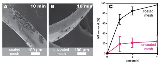
Fig. 2 SEM images of P EH dip-coated stainless-steel mesh (A) and uncoated stainless-steel mesh (B) after 10 min of a capture experiment. (C) Plot of microplastic removal efficiencies (percent removed relative to a control) versus time (min), as quantified by flow cytometry. All capture experiments were performed in 80/20 water/ethanol solutions containing 500 mg L -1 of PS microplastics (10 μm diameter).
