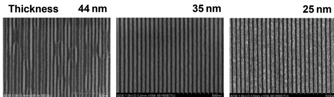
Fig. 2 SEM images of 25 nm L/S patterns (top view) for the PSNA 0.4 resist at different film thicknesses (exposure doses: 1600, 1415 and 1126 \mu\text{C cm}^{-2} ).
