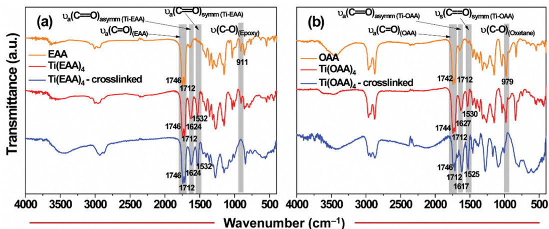
Fig. 2 Probing of metal chelation and ring opening polymerization in (a) \text{Ti}(\text{EAA})_4 and (b) \text{Ti}(\text{OAA})_4 resin formulations through FT-IR analyses.
