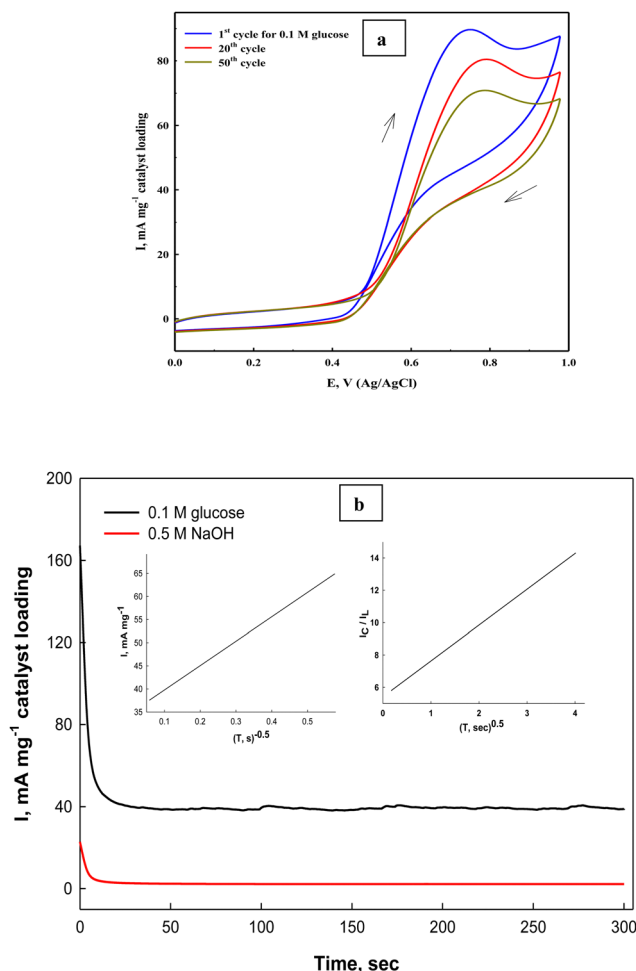
Fig. 12 (a) Repeated cyclization of the Ni(II)-SB/C electrode in 0.5 M NaOH + 0.1 M glucose, and (b) chronoamperometry of the same electrode at 0.72 V and the inset plots represent I and 1/\sqrt{t} (left) and the relationship of I_C/I_L and square root of time (right).
