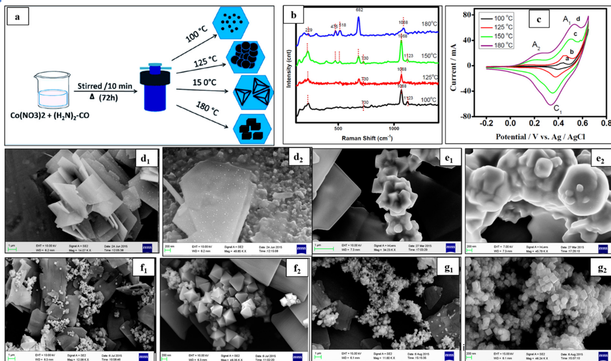
Fig. 12 (a) Schematic illustration of the synthesis process and the resulting structures. (b) Raman shift and (c) CV of all synthesized samples at 50 \text{ mV s}^{-1} . Low and high magnification images of the \text{Co}_3\text{O}_4 electrode obtained at (d 1 ) and (d 2 ) 100^\circ\text{C} , (e 1 ) and (e 2 ) 125^\circ\text{C} , (f 1 ) and (f 2 ) 150^\circ\text{C} , and (g 1 ) and (g 2 ) 180^\circ\text{C} . Reproduced with permission from ref. 161. Copyright 2017 MDPI publications.
