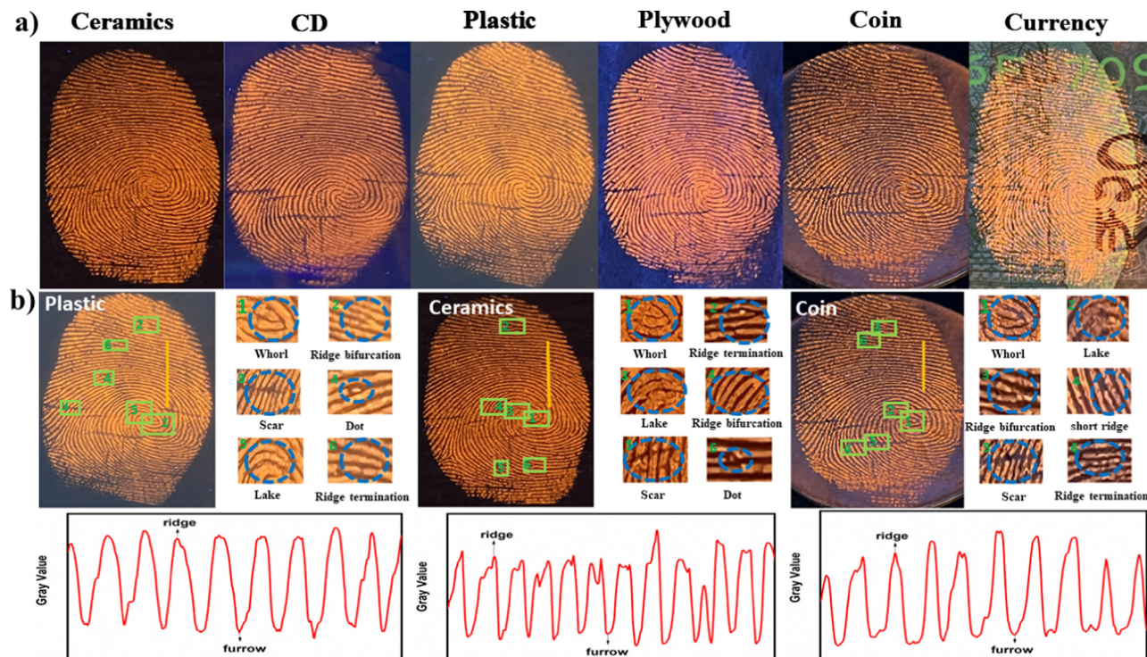
Fig. 6 (a) LFM developed on various substrates such as ceramics, CDs, plastic, plywood, coins, and currency; (b) level 1, level 2 and level 3 details of the developed LFM on plastic, ceramics and coins and the variations of the fluorescence intensity between the fingerprint ridges and furrows across the yellow line.
