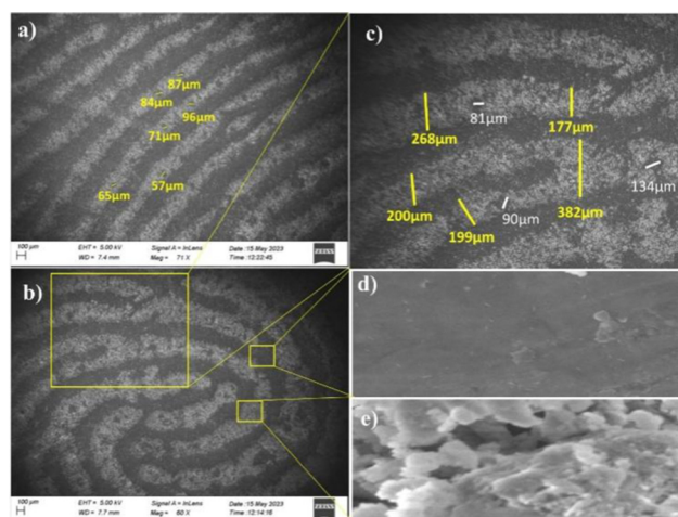
Fig. 7 The micromorphology of LFM was characterized by FE-SEM; (a) super-resolution of the LFM ridge pattern (insets: yellow-pore size); (b) whorl image; (c) magnified image of a whorl (insets: yellow-ridge width, white lake width); (d) furrow area; (e) ridge area.
