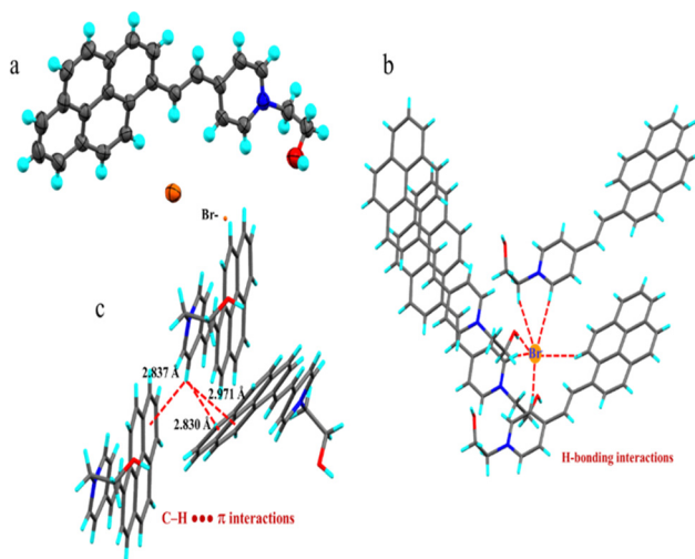
Fig. 4 (a) Molecular structure of the Py-Pr-OH ; (b) H-bonding interactions involving various protons with a central \text{Br}^- ion; (c) C–H \cdots \pi interactions in the Py-Pr-OH molecule.
