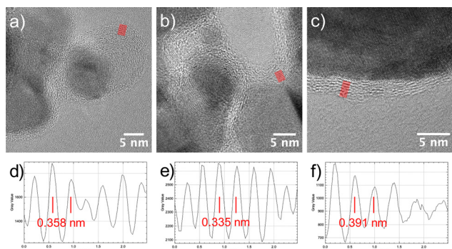
Fig. 5 (a)–(c) HRTEM images evidencing the presence of graphitic carbon layer on \text{Ni}_3\text{C} and \text{NiC}_7 particles recovered after 2 h of \text{H}_2 –Ar plasma exposure of the turbostratic disordered \alpha -hydroxide powder. (d) and (f) Intensity profiles corresponding to the red lines in (a)–(c); the deduced mean interplanar distances are indicated.
