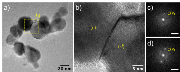
Fig. 4 (a) TEM bright field image of \text{Ni}_3\text{C} and \text{NiC}_7 particles attached to each other. (b) HRTEM image of the area labelled (b) in image (a) showing the grain boundary between the \text{Ni}_3\text{C} particles. From the FFT analyses shown in (c) and (d), it can be deduced that the {001} planes of both the crystals are parallel, and d_{006} was found to be 2.17 \pm 0.01 \text{ \AA} , in agreement with the calculated value using the cell parameters inferred from the XRD analysis (Table S1, ESI†). Scale bar on (c) and (d) is 0.5 \text{ \AA}^{-1} .
