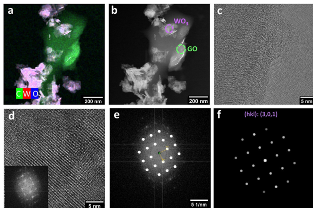
Fig. 5 (a) HAADF-STEM micrograph of \text{WO}_3\text{GO}_{200\text{ }^\circ\text{C-10 min}} with the elemental map obtained from \text{W}_{L_{23}} , \text{O}_{K_{\alpha}} , and \text{C}_{K_{\alpha}} . (b) HAADF image with selected regions of \text{WO}_3 and GO and (c) HRTEM images of GO and (d) \text{WO}_3 with a fast-Fourier-transform pattern (FFT – inset). (e) FFT pattern fitted with the schematic diagram of monoclinic \text{WO}_3 (301) and (f) calculated diffraction pattern (301).
