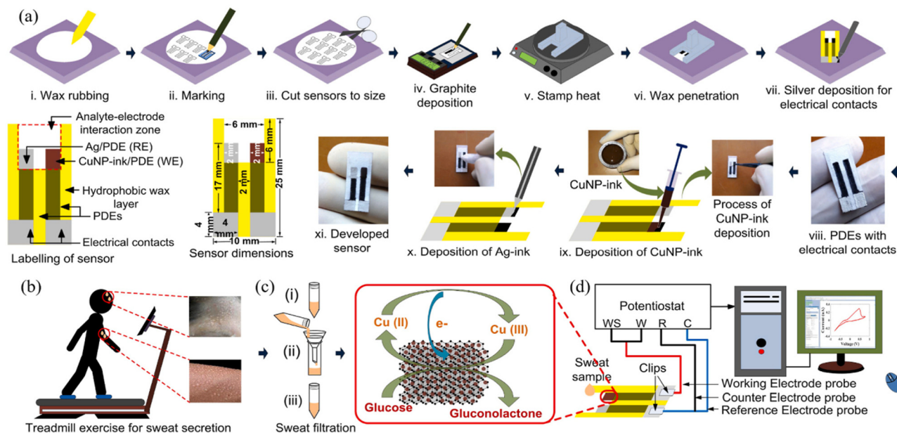
Fig. 5 (a) Schematic of the design and manufacture of two-electrode enzyme-free human sweat glucose sensor (i–xi) with the sensor dimensions and labelling, (b) secretion of sweat during treadmill exercise at room temperature, (c) filtration of sweat, and (d) set-up for developed sensor connected to a potentiostat with a computer system for detecting the level of sweat glucose in a human sweat sample. Reproduced with permission from ref. 150 Copyright 2022, Elsevier.
