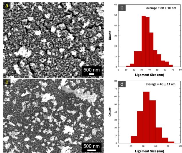
Fig. 6 (a) SEM micrograph of np-CuSn on GC substrate at magnification of 50 000 \times and the respective ligament size distribution (b); (c) SEM micrograph of np-CuSn on Cu substrate at 30 000 \times magnification and the respective ligament size distribution (d).
