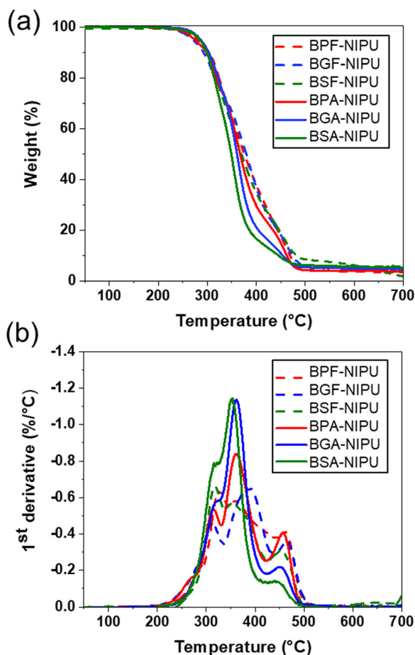
Fig. 4 (a) TGA thermograms of NIPUs in N_2 atmosphere; sample weight (%) as a function of temperature with a heating rate of 10 °C min^{-1} , and (b) the first derivative of the weight remaining ( \%/^{\circ}C ) as a function of temperature for all NIPUs.
