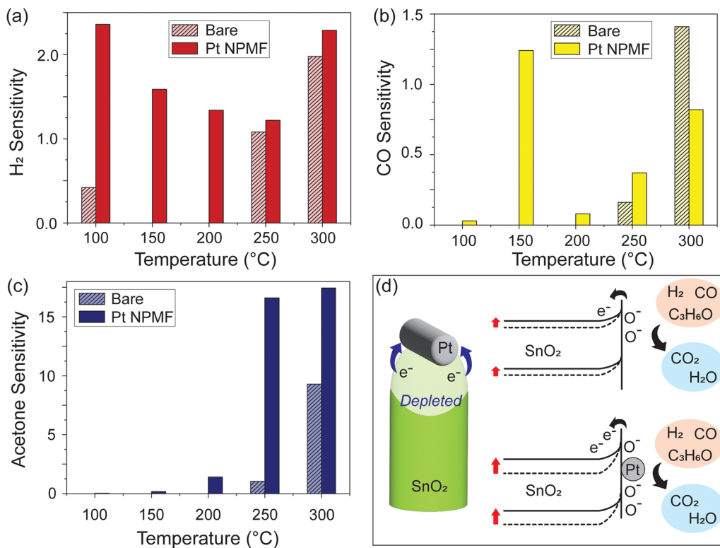
Fig. 5 Sensitivity as a function of the operating temperature and role of Pt NPMF: (a) H 2 , (b) CO, and (c) Acetone sensitivity for the bare device (striped) and Pt NPMF transferred device (filled). Pt NPMF transferred device clearly shows enhanced sensitivity for three gases, especially at lower temperature. (d) Sensing mechanism comparison for SnO 2 nanostructures with (bottom) and without (top) Pt NPMF coating. Top: Electron concentration in SnO 2 increases upon gas exposure as gases donate electrons through chemical reactions. Bottom: Pt NPMF enhances electron depletion via the Schottky effect and catalyzes additional electron donation upon gas exposure, significantly affecting electron concentration modulation in SnO 2 .
