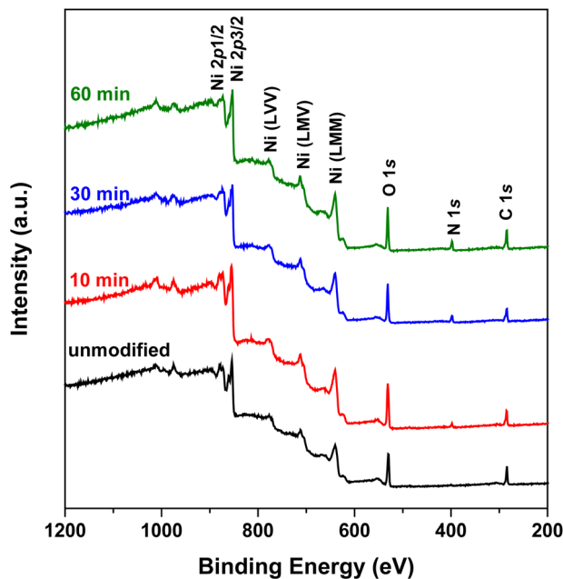
Fig. 4 XPS survey spectra of the unmodified and N_2 plasma-modified Ni foam electrodes.
