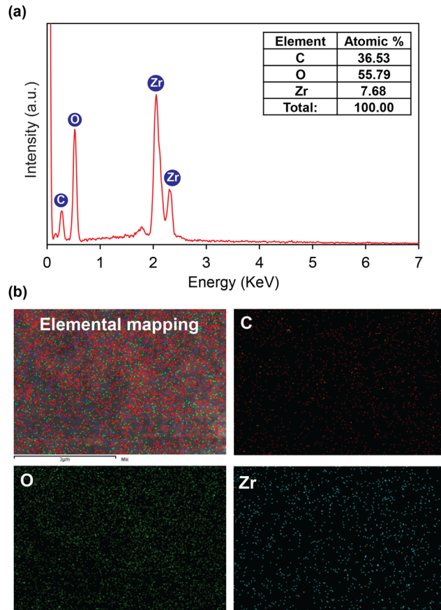
Fig. 3 EDX spectrum of activated HCMUE-2 (a); elemental mapping by SEM-EDX of activated HCMUE-2 (b).
