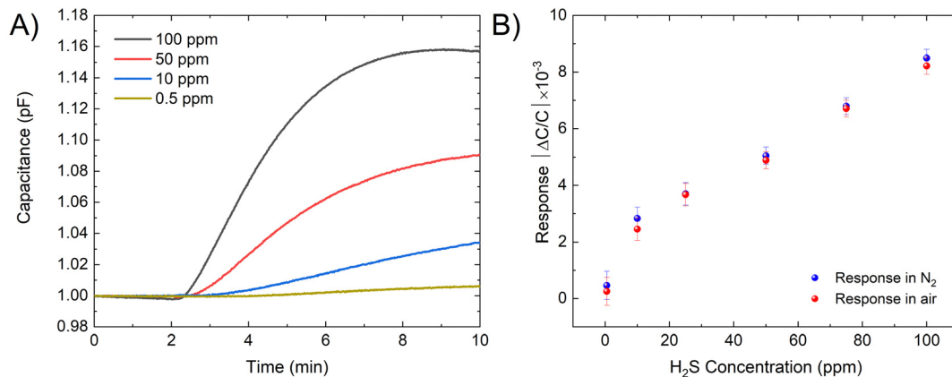
Fig. 2 (A) Capacitive sensor response for kag -MOF in the presence of different concentration of \text{H}_2\text{S} . (B) The response of the sensor for different \text{H}_2\text{S} concentrations.
