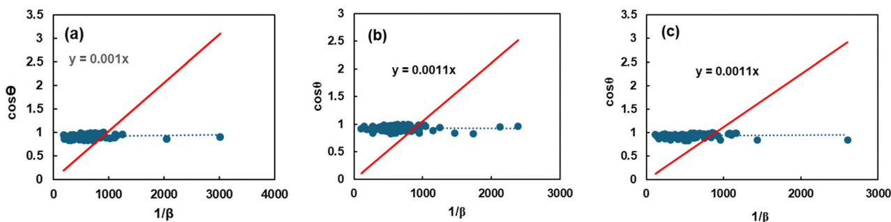
Fig. 9 Graphical representation of the Sahadat–Scherrer model to calculate the crystallite properties of TSP from (a) Turrítella, (b) Cardium, and (c) Conch shells.
