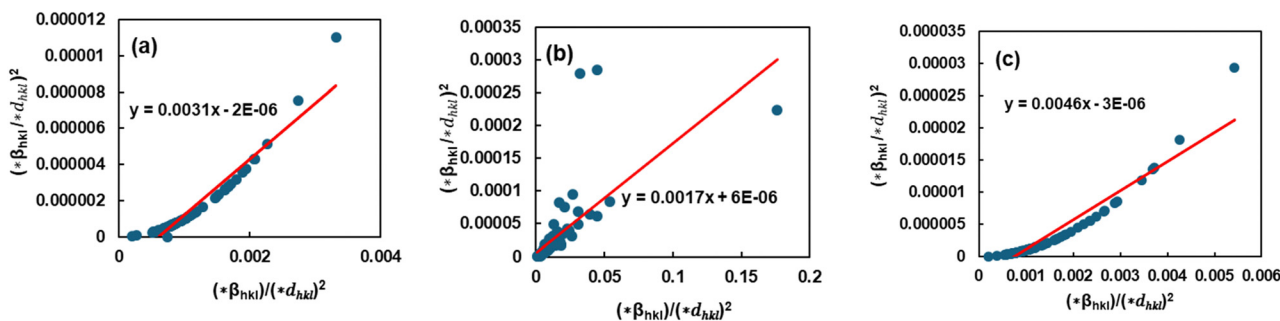
Fig. 8 Graphical illustration of the Halder–Wagner model to estimate the crystallite properties of TSP from (a) Turrítella, (b) Cardium, and (c) Conch shells.
