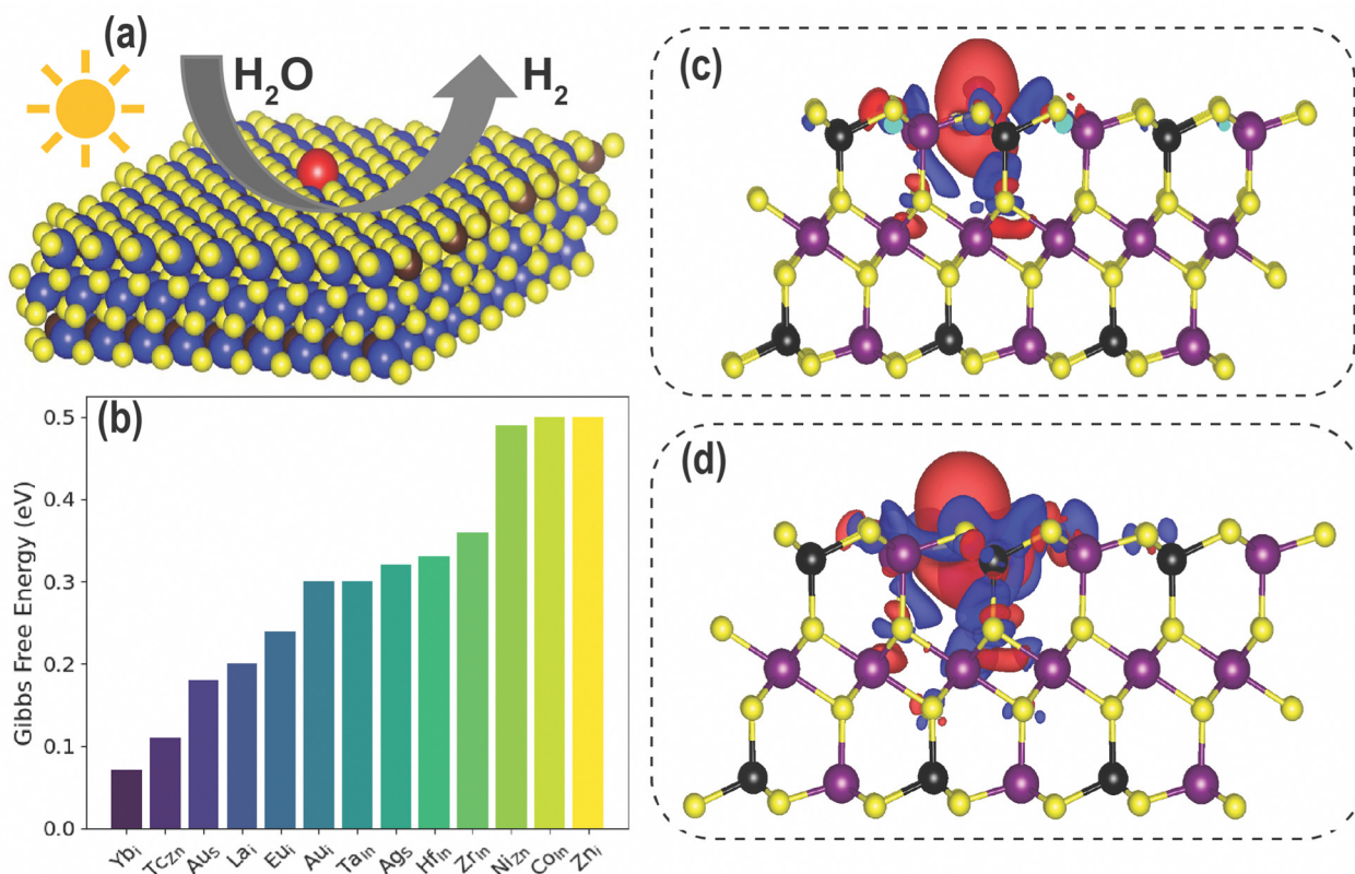
Fig. 6 (a) Illustration of the photocatalytic HER on the surface of SAC doped ZIS (b) comparison of Gibbs free energy ( \Delta G ) for pristine ZIS, and screened SACs such as Co_{In} , Yb_i , TC_{Zn} , Au_S , La_i , Eu_i , Ag_S , Au_i , Ta_{In} , Hf_{In} , Zr_{In} , Ni_{Zn} and charge density difference (CDD) analysis of (c) ZIS and (d) Yb_i system.
