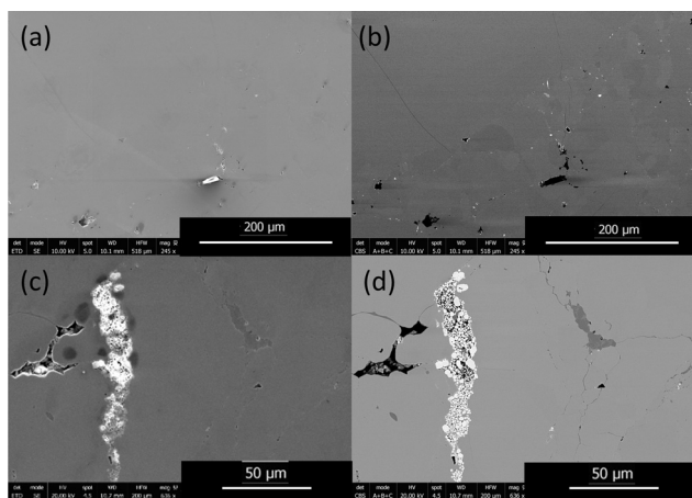
Fig. 2 (a) and (b) The secondary electron (SE) image and back-scattered electron (BSE) image of the \text{YbZn}_{11} sample at a larger scale (with a scale bar of 200 \mu\text{m} ) at the same site. The bright feature shown in SE image (a) is charging from a glass fragment coming from the synthesis process, which can be confirmed by the fact that the BSE image shows a low electron count from back-scattering, indicating low mass elements. (c) and (d) SE and BSE images at higher magnification (scale bar of 50 \mu\text{m} ) on typical defects.
