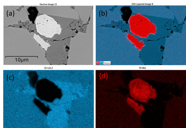
Fig. 3 EDS mapping. (a) BSE image of a typical defect site with cavities (black), Yb oxides (white), Zn (dark grey), and compared to \text{YbZn}_{11} (light grey). (b) layered EDS map, (c) Zn distribution EDS map, and (d) Yb distribution map. The blue and red dots in (c) and (d) represent the relative Zn and Yb concentration.
