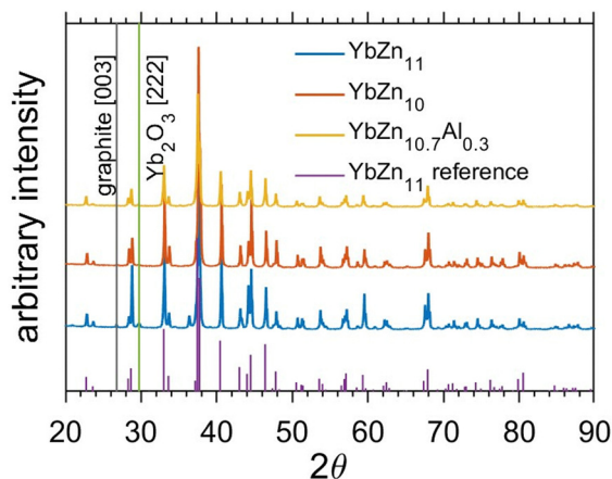
Fig. 1 XRD results of Yb–Zn samples, the annealed intrinsic \text{YbZn}_{11} sample in blue, the Zn-deficient sample \text{YbZn}_{10} sample in orange, and the Al-substitution sample \text{YbZn}_{10.7}\text{Al}_{0.3} in yellow, and the reference peaks in purple. 28 Minor impurity peaks from graphite and ytterbium oxide are marked by black and green lines.
