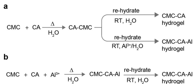
Scheme 1 (a) Synthesis of mono-cross-linked CMC–CA hydrogel and dual-cross-linked CMC–CA–Al hydrogels obtained by the sequential addition of cross-linkers, i.e. , CA is added first and then the gels are soaked in \text{Al}^{3+} solution. (b) Synthesis of dual-cross-linked CMC–CA–Al hydrogels obtained by the simultaneous addition of cross-linkers CA and \text{Al}^{3+} at the beginning of the gelation process. Both methods provided stable hydrogel films: see Fig. S1, ESI† for the chemical structures and photographs of the resulting hydrogels.
